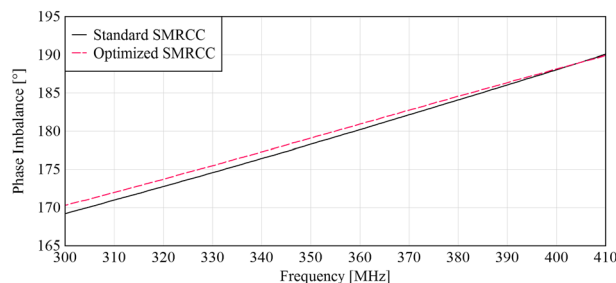
Figure 5. Simulated (HFSS) phase imbalance of the standard SMRRC and of the optimized 180° hybrid proposed in this paper.
