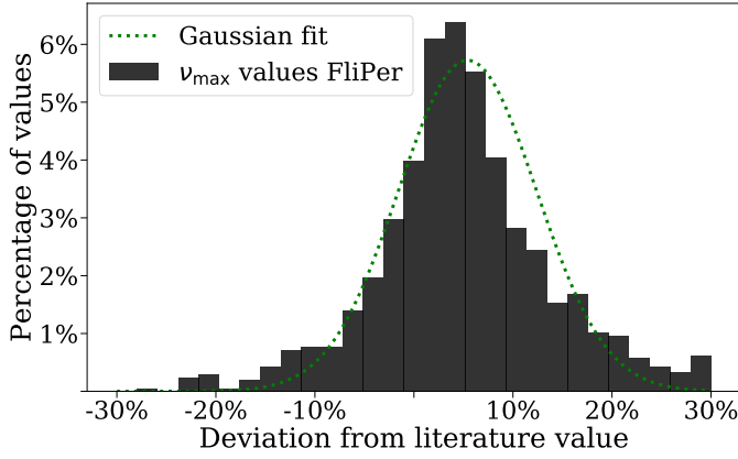
Fig. 2. Distribution of values for \nu_{\max} extracted from the FliPer method. The Y axis shows the percentage of values within a given bin of deviation from a corresponding literature value, while the X axis shows the deviation from the literature value in percent. The distribution can be represented by a Gaussian function, whose fit to the histogram is represented by a dotted green line. The mean for this distribution is at 4.95%, with a standard deviation of 6.93%. For visualisation purposes, deviations above 30% and below -30% are excluded.
