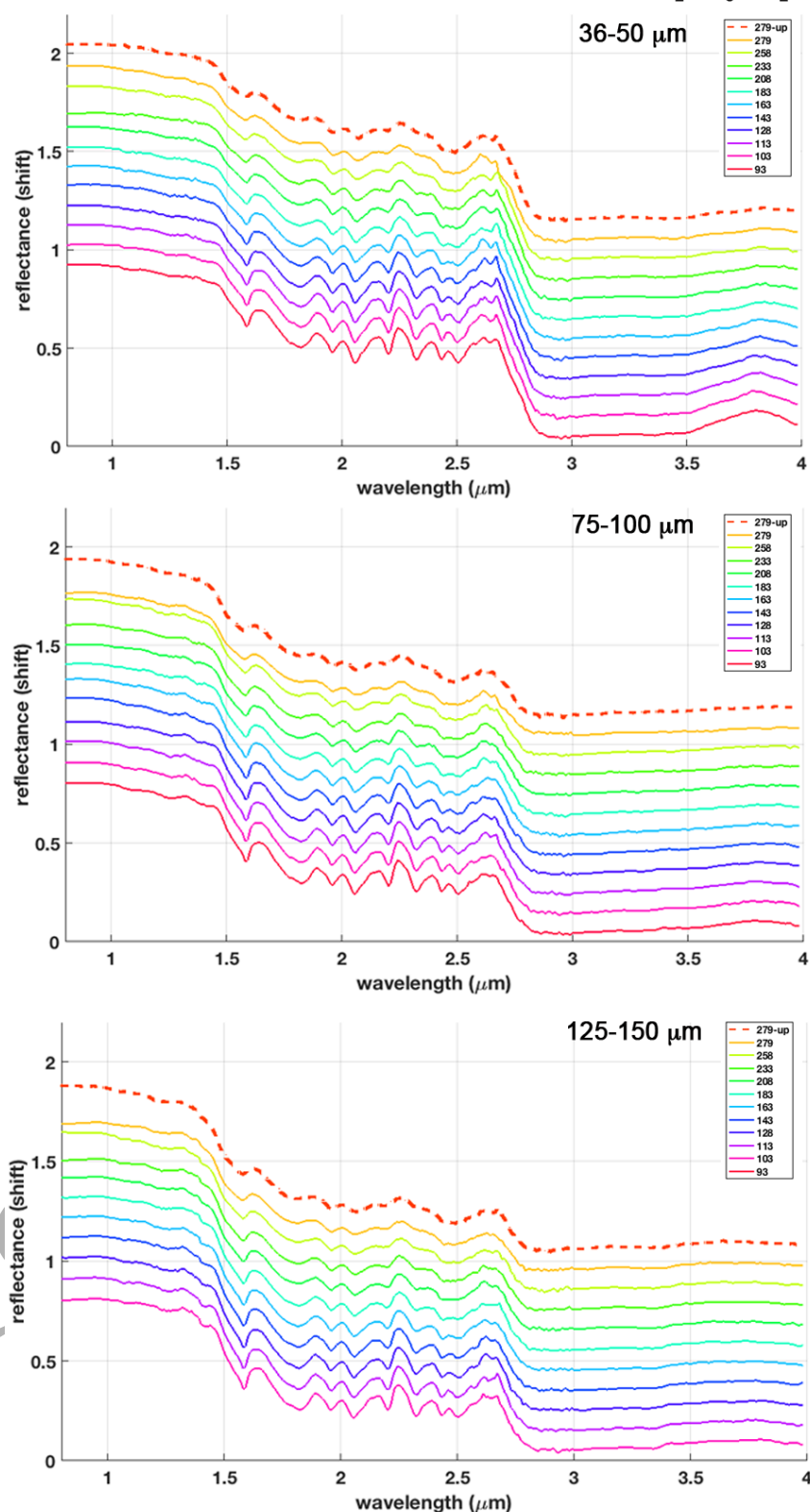
Figure 2. Spectra of monohydrated sodium carbonate ( \text{Na}_2\text{CO}_3 \bullet \text{H}_2\text{O} ) acquired at different temperatures in the range 93-279 K. Measurements at 279 K have been acquired both at the beginning and at the end of the sequence. An arbitrary offset of 0.1 in reflectance is applied to all spectra for clarity. For the 125-150 \mu\text{m} grain size the T=113 K spectrum has not been measured. The bottommost spectrum corresponds to the true reflectance value, \approx 0.9 at 1 \mu\text{m} .
