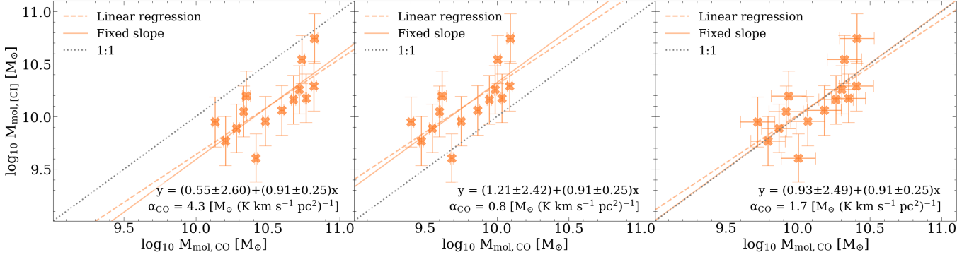
Fig. 4. [CI]-based M_{\text{mol}} vs. CO-based M_{\text{mol}} values obtained with different \alpha_{\text{CO}} assumptions ( 0.8, 4.3 , and 1.7 M_{\odot} (\text{K km s}^{-1} \text{pc}^2)^{-1} ). The best-fit linear relation with a free-varying slope is shown as a dashed orange line, and the best-fit parameters are reported at the bottom-right corner of each plot. The solid orange line shows the best-fit relation obtained by fixing the slope to unity, and the 1:1 relation is reported as a dotted black line.
