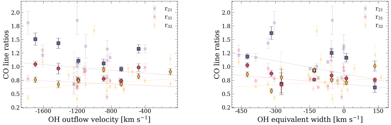
Fig. 11. Global CO line ratios as a function of \text{OH}_{\text{max}} (left) and \text{OH}_{\text{EQW}} (right) for the sources with OH119 \mu\text{m} data as reported in the literature (see Table 1). The binned values (computed in the same way as in Sect. 5.4) are shown using darker colors and overplotted on the individual data points. Dashed lines indicate the best-fit relations obtained from a least squares regression analysis conducted for each transition line separately. The color coding refers to different line ratios, as indicated in the legend at the top-right corner of each plot.
