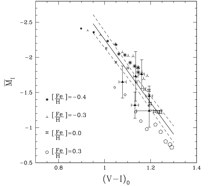
FIG. 7.— \bar{M}_I vs. (V - I)_0 . Symbols are as in Fig. 5. In the figure we plot the calibration from Jensen et al. (2003; solid line), and 1\sigma dispersion lines are reported with the dashed line. A sample of shell elliptical galaxies from Tonry et al. (2001) are reported as triangles. The absolute SBF magnitudes are derived coupling the apparent SBF measurements, with the SBF-independent DMs reported in Table 4. It is noticeable the absence of any systematic deviation of shell ellipticals with respect to the empirical calibration ( \langle \bar{M}_{J03} - \bar{M}_{\text{non-SBF DMs}} \rangle = -0.06 \pm 0.22 ), and to the stellar population models.
