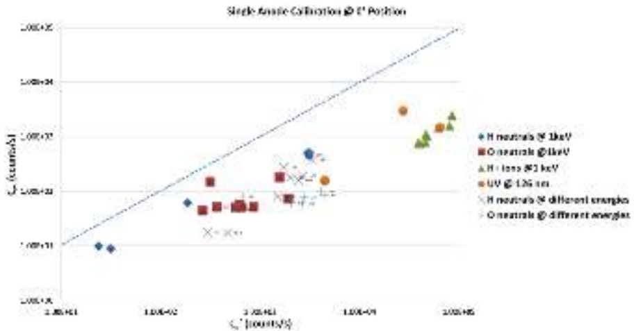
Fig. 49 Expected counts at 0^\circ angle to the normal for different flux intensities, energies, species and charges vs real counts at the peak sector. Comparison with the 1 by 1 curve (dashed line)
