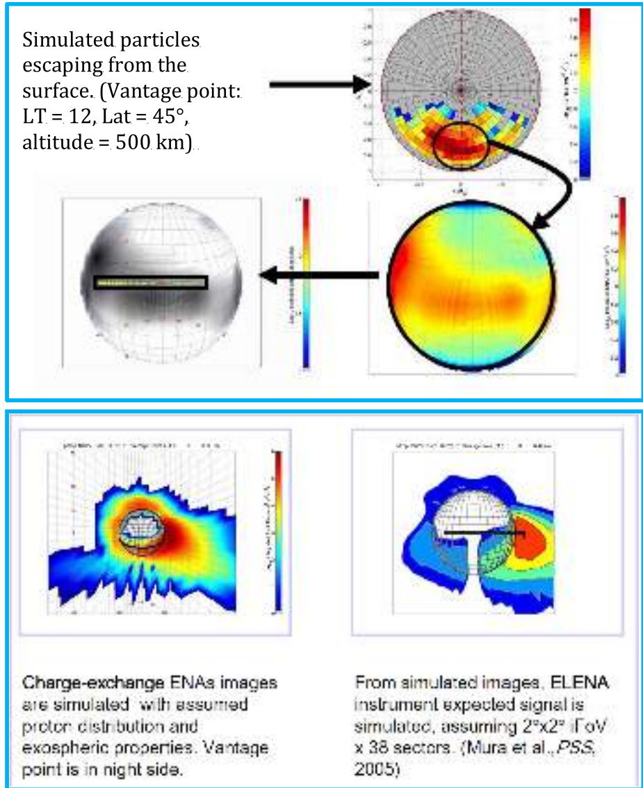
Fig. 18 Upper: Simulation of the energy-integrated (between 20–1000 eV) signal from vantage point MLT=1200, 45° elevation and 500 km altitude is shown in the upper panel. The horizon at this position is zoomed in the bottom-right panel and the slice of ELENA FOV is evidenced in the bottom-left panel. Bottom: Energy-integrated H ENA from the night side apoherm (left panel). The instantaneous FOV of the linear array of the ELENA sensor is shown as a slice in the right panel (from Mura et al. 2005, 2006)
