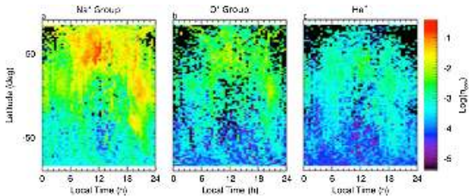
Fig. 4 \text{Na}^+ -group (a), \text{O}^+ -group (b), and \text{He}^+ (c) ion observed density along the MESSENGER orbit as a function of local time and planetary latitude (note that the northern data refer to lower altitudes). Observed regions with zero counts are colored black (Raines et al. 2015)
