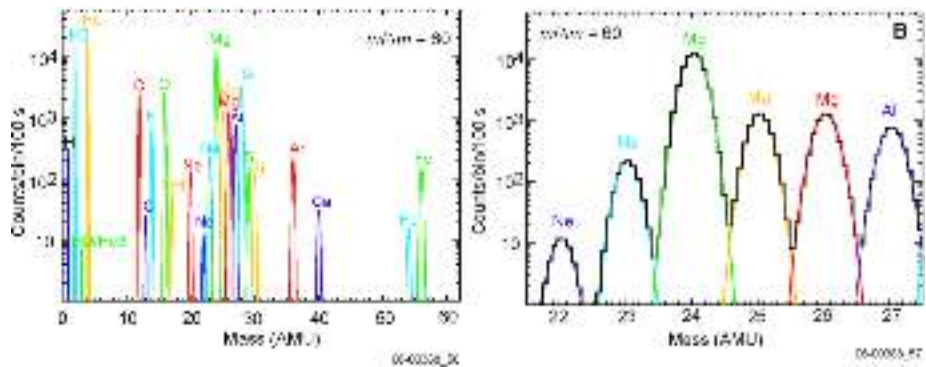
Fig. 21 Expected Strofio performance at Mercury. Both elements and isotopes will be resolved in Mercury's exosphere
