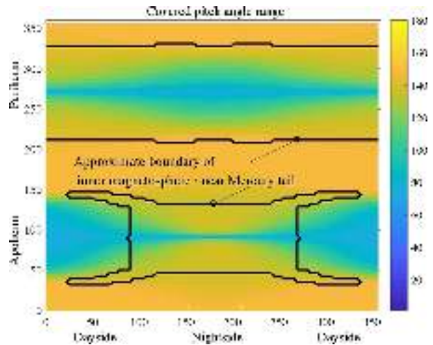
Fig. 27 The pitch-angle range covered by MIPA as a function of the beta-angle and true anomaly angle. (0, 0) corresponds to the noon-midnight orbit with the pericenter at the subsolar point
