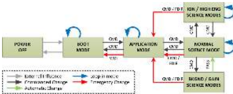
Fig. 87 Strofiu Mode Transition Diagram
