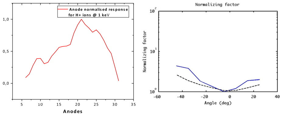
Fig. 48 ( left ) Normalized angular scan counts for 1-keV \text{H}^+ . ( right ) Observed sector normalization factors for 1-keV O (blue line), and theoretical curve of the normalization factor (dashed black line)
