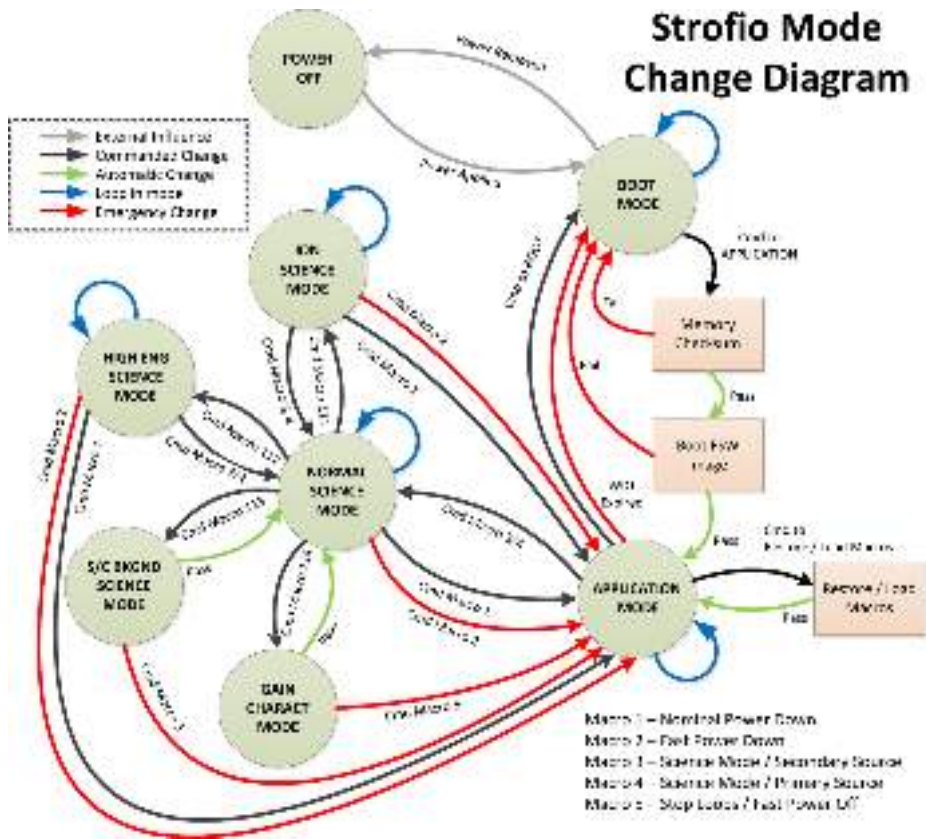
Fig. 86 Strofi State Diagram
