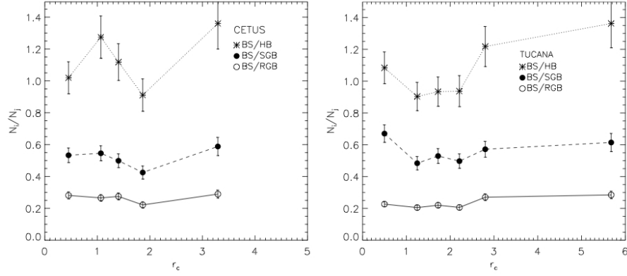
Fig. 6.6 The BSS radial distribution as a function of the core galacto-centric radius for the Cetus (left) and Tucana (right) dwarf galaxies. The absence of a central peak points to the lack of collisional BSS in dwarf galaxies. This figure is reproduced from [52] with permission by the AAS.
