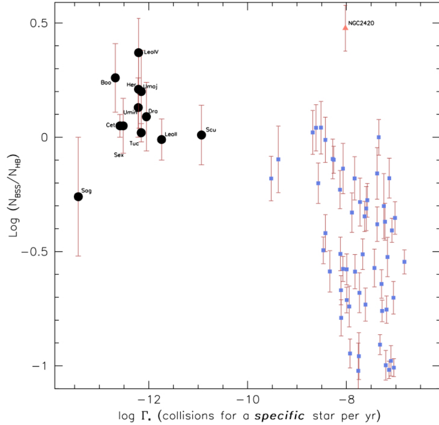
Fig. 6.5 The BSS frequency as a function of the stellar collision factor for a specific star per year. Globular clusters are plotted as filled squares, while dwarf galaxies are plotted as filled circles. The filled triangle is that of an open cluster.
