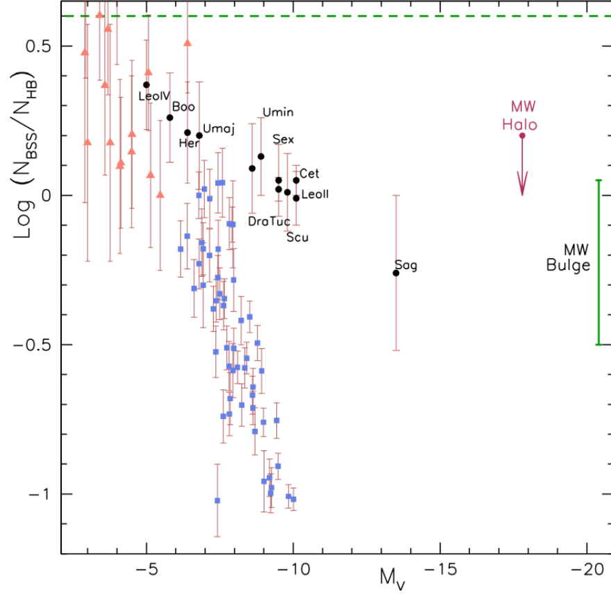
Fig. 6.4 The BSS frequency ( F_{HB}^{BSS} ) vs M_V diagram for globular clusters [56], open clusters [14], and dwarf galaxies [50]. The horizontal line shows the mean BSS frequency as derived for the Milky Way field stars by [60]. The range of the BSS frequency for the Milky Way Bulge [11] is shown as a bar at M_V = -20.4 . A preliminary upper limit for the Milky Way Halo BSS frequency (as normalised to only the blue horizontal branch stars) is shown at M_V = -17.8 .
