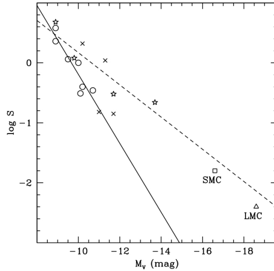
Fig. 6.10 The Anomalous Cepheid frequency ( \log S , per 10^5 L_\odot ) as a function of the M_V of the parent dwarf galaxy (i.e. the ACs frequency– M_V anti-correlation). Open circles highlight purely ancient galaxies while starred symbols indicate galaxies with large intermediate-age populations. The solid line shows an excellent fit to only the ancient systems (included in this review). This figure is reproduced from [19] with permission by Astronomy & Astrophysics, © ESO.
