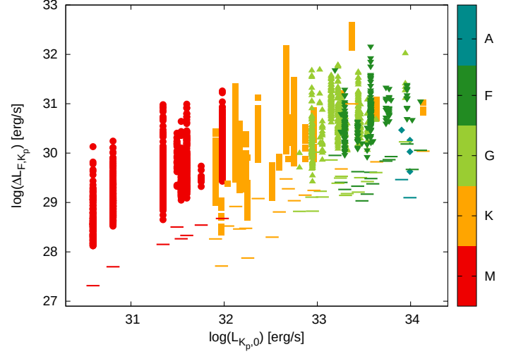
Fig. 14: Absolute flare amplitudes versus quiescent luminosity represented by the Kepler magnitude associated with the ‘flat-tened’ lightcurve; see text for details.
