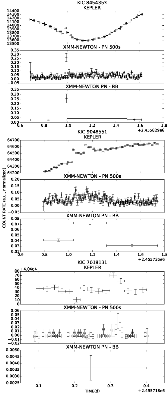
Fig. 8: Simultaneous Kepler and XMM-Newton EPIC PN light curves for the stars showing a simultaneous X-ray and white-light flare. The EPIC light curves produced by the EXTrAS pipeline with 500 s uniform binning and with the bayesian blocks adaptive binning are plotted. The flare in the Kepler light curve of KIC 7018131 corresponds to a bump in the EPIC uniform bin lightcurve which is, however, not significant at a 3\sigma level over the baseline, and not detected with the bayesian block algorithm.
