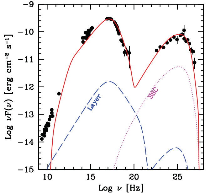
Figure 7. As Fig. 2. Lines show the results of the structured jet model. The dashed blue line shows the emission from the layer. The magenta dotted line reports the SSC emission from the spine. See text for details.
