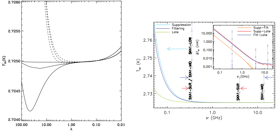
Fig. 1. Left panel: distorted spectra in equivalent thermodynamic temperature vs. \lambda (cm) with late energy injection \Delta\epsilon/\epsilon_i \simeq 4y = 5 \times 10^{-6} plus an early/intermediate energy injection \Delta\epsilon/\epsilon_i = 5 \times 10^{-6} ( \sim 20 times smaller than current upper limits) at the “time” Comptonization parameter y_h = 5, 1, 0.01 (bottom to top; the cases at y_h = 5 and 1 are very similar at short \lambda ; solid lines) plus a FF distortion with y_B = 10^{-6} (dashes). y_h = y , but assuming electron temperature equal to the radiation one and computing the integral from the energy injection time to the current time. Right panel: FF distortion in SKA2 frequency range by two astrophysical reionization histories (a late phenomenological model is also displayed for comparison). Inset: models absolute differences; vertical lines: ranges of SKA1 configurations. From Ref. 2.
