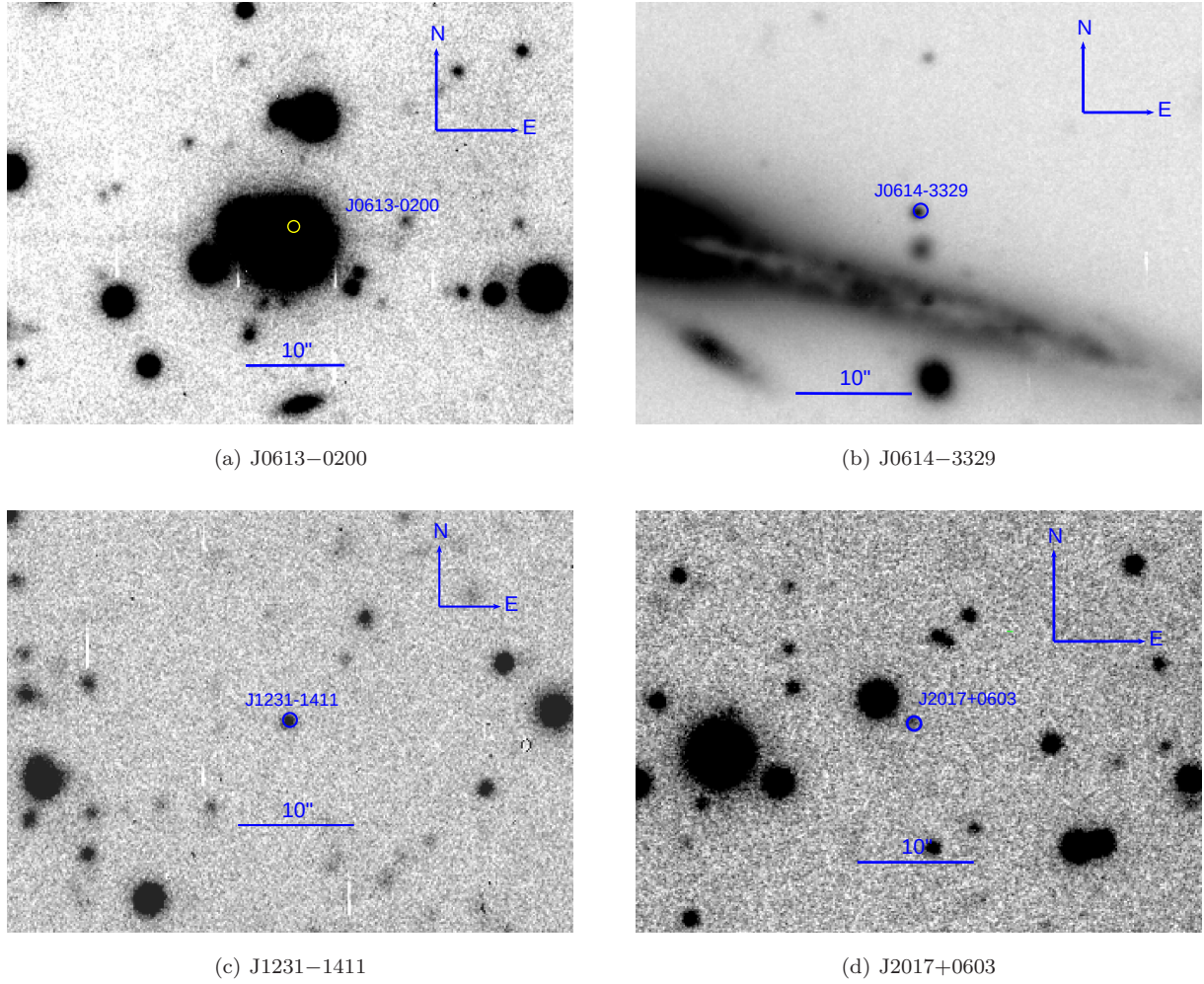
Figure 1. GMOS r-band images of the four MSP fields. The circles correspond to the computed MSP radio positions. Since the error on the radio coordinates is below 1 mas (see Table 1) the uncertainty on the computed radio position is dominated by the accuracy our astrometry calibration (0''.2; Sectn. 3.2). The circle radius corresponds to three times such an uncertainty for a better visualisation. For the other pulsars, the companion stars are marked by the ticks and labelled by the pulsar names. PSR J0614-3329 is located a few arcsec north of the disk of the bright galaxy ESO 365-1 (Lauberts & Valentijn 1989). All images have been obtained from the co-addition of all r-band science frames, apart from the PSR J0613-0200 one which has been obtained from the co-addition of short exposures only to avoid saturation of the bright star near the pulsar position.
