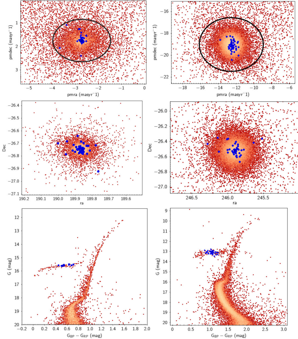
Figure 3. Proper motions (top), spatial distribution (middle) and G , G_{BP} – G_{RP} colour–magnitude diagram (CMD; bottom) of two GCs in our sample: NGC 4590 ( [Fe/H] = -2.27 ; left) and NGC 6121 ( [Fe/H] = -1.18 ; right). The CMDs are drawn using for constant stars magnitudes from the EDR3 catalogue. Black ellipses in the top panels encircle stars plotted in the CMDs in the bottom panels of the figure. Blue dots show the cluster RRLs (42 RRLs in the top and middle panels and 13 RRLs with mean G , G_{BP} , and G_{RP} magnitudes from the Gaia DR2 vari_rrlyrae table, in the CMD of NGC 4590; 47 RRLs in the top and middle panels and 37 RRLs in the CMD of NGC 6121).
