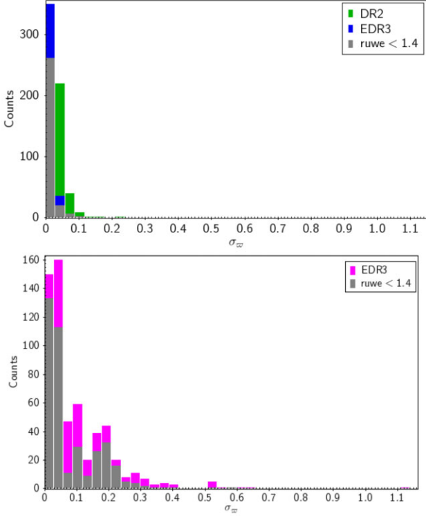
Figure 2. Top panel: The blue histogram shows the distribution of the EDR3 parallax uncertainties ( \sigma_{\text{EDR3}} ) for our initial sample of 397 field RRLs. For comparison the DR2 parallax uncertainties of the stars are represented by a green histogram. The grey histogram shows the \sigma_{\text{EDR3}} distribution for the subsample of 291 RRLs with \text{ruwe} < 1.4 . Bottom panel: The magenta histogram shows the distribution of the EDR3 parallax uncertainties for our initial sample of 582 RRLs in GCs. The grey histogram shows the \sigma_{\text{EDR3}} distribution for the subsample of 385 GC RRLs with \text{ruwe} < 1.4 . In both panels, the bin size is 0.03 mas.
