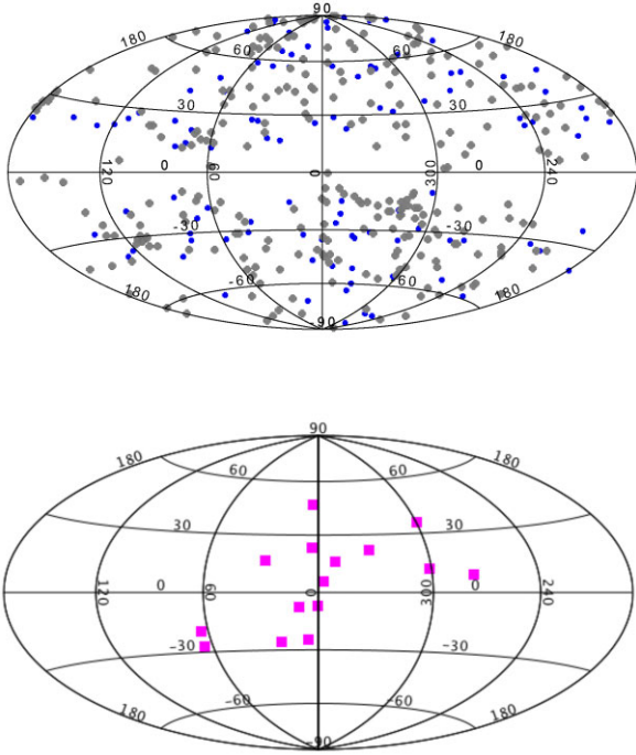
Figure 1. Top panel: Hammer–Aitoff projection in galactic coordinates of the sky distribution for the sample of 397 Galactic field RRLs and the subsample of 291 RRLs with ruwe < 1.4 (blue and grey symbols in the upper plot, respectively). Bottom panel: The 15 globular clusters (magenta symbols, lower plot) hosting the RRLs considered in this study.
