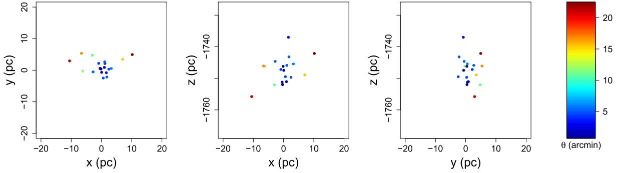
Figure 13. Spatial distribution inferred by our PW_{(G, G_{BP}, G_{RP})}Z HM for 20 RRLs in NGC 6121 projected on to the coordinate planes associated with the reference frame described in the text. The colour scale encodes the angular separation between the RRLs and the cluster centre. Posterior credible intervals are omitted for clarity, but along the z -axis (line of sight) are of the order of 100 pc.
