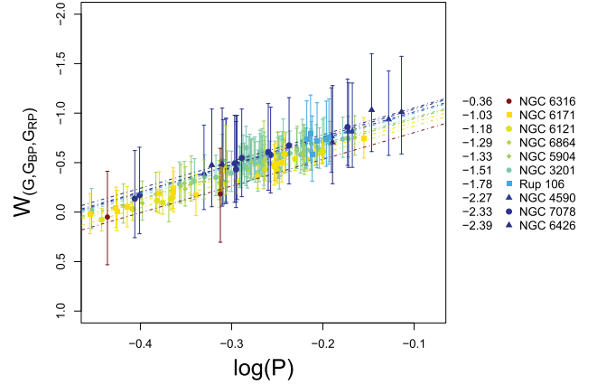
Figure 10. Wesenheit magnitudes inferred by the HM as a function of the decadic logarithm of the true period. The dashed lines represent the P W(G, G_{BP}, G_{RP}) relations of equation (5) particularized for the parameters of Table 6. Colours encode the true metallicity of each globular cluster on the Carretta et al. (2009) metallicity scale according to the scale on the right.
