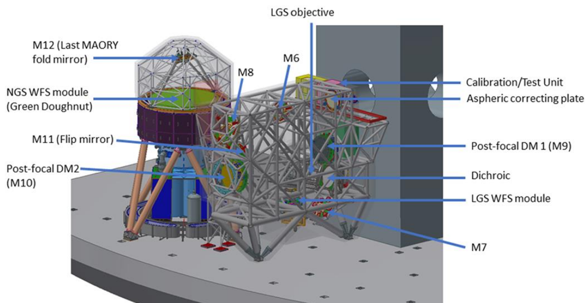
Figure 2. MORFEO sub-systems and main components
