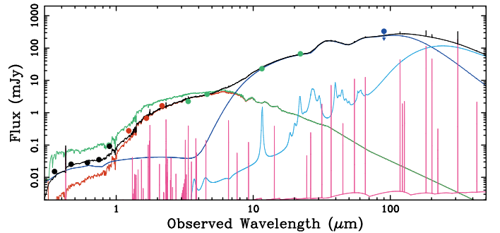
Fig. 3. SED fitting of WISE J1042+1641. Filled circles represent the observational data from the SDSS (black), 2MASS (red), and WISE (green). The 5\sigma upper limit from AKARI is denoted as a blue arrow. The best-fit SED is denoted with the black solid line. Different components are also shown: unattenuated stellar emission (green line), attenuated stellar emission (red line), nebular emission (pink line), SF-heated dust emission (light blue line), and AGN emission (blue line).
