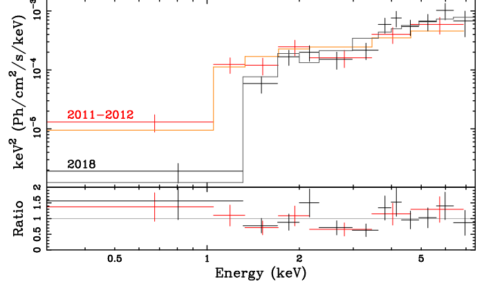
Fig. 2. Swift /XRT spectra in 2011–2012 (red) and in 2018 (black), with their best-fit absorbed pexmon model shown as orange and dark gray lines, respectively ( top panel ) and the data-model ratios ( bottom panel ). They are corrected for the effective area of the instrument and are given in units of E F_E ( F_E is the energy flux at the energy E ).
