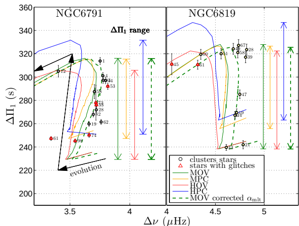
Figure 1. Red-clump stars in NGC6791 and NGC6891 in a \Delta\Pi_1 - \Delta\nu diagram. Model predictions based on different near-core mixing schemes are shown by solid lines. The vertical lines indicate the range of \Delta\Pi_1 covered by each mixing scheme. The dashed line shows MOV models computed with slightly ( \lesssim 3\% ) increased mixing-length parameters (compared to the solar-calibrated value). The red triangles mark the presence of buoyancy glitches which, to the first order, induce a modulation in \Delta\Pi_1 with respect to the asymptotic value (Miglio et al. 2008, Cunha et al. 2015, and Fig. 10 of Mosser et al. 2015), potentially hampering an accurate inference of the asymptotic \Delta\Pi_1 .
