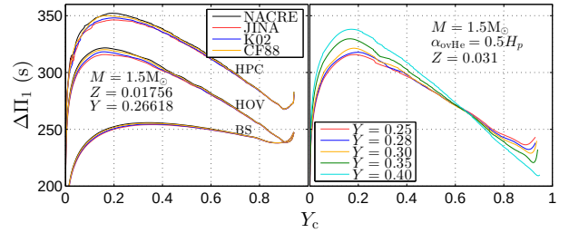
Figure 4. Left panel: RC- \Delta\Pi_1 evolution as a function of central helium mass of a M = 1.50 M_\odot solar metallicity star with three different mixing schemes and four different ^{12}\text{C}(\alpha,\gamma)^{16}\text{O} reaction rates. Right panel: RC- \Delta\Pi_1 evolution as a function of central helium mass fraction of a M = 1.50 M_\odot star computed assuming three different combinations of Z and Y .
