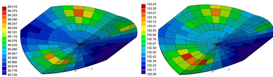
Fig. 24 VG2 thermal gradient in the Cold (left) and Hot (right) cases. Temperature is expressed in the absolute scale (K)
