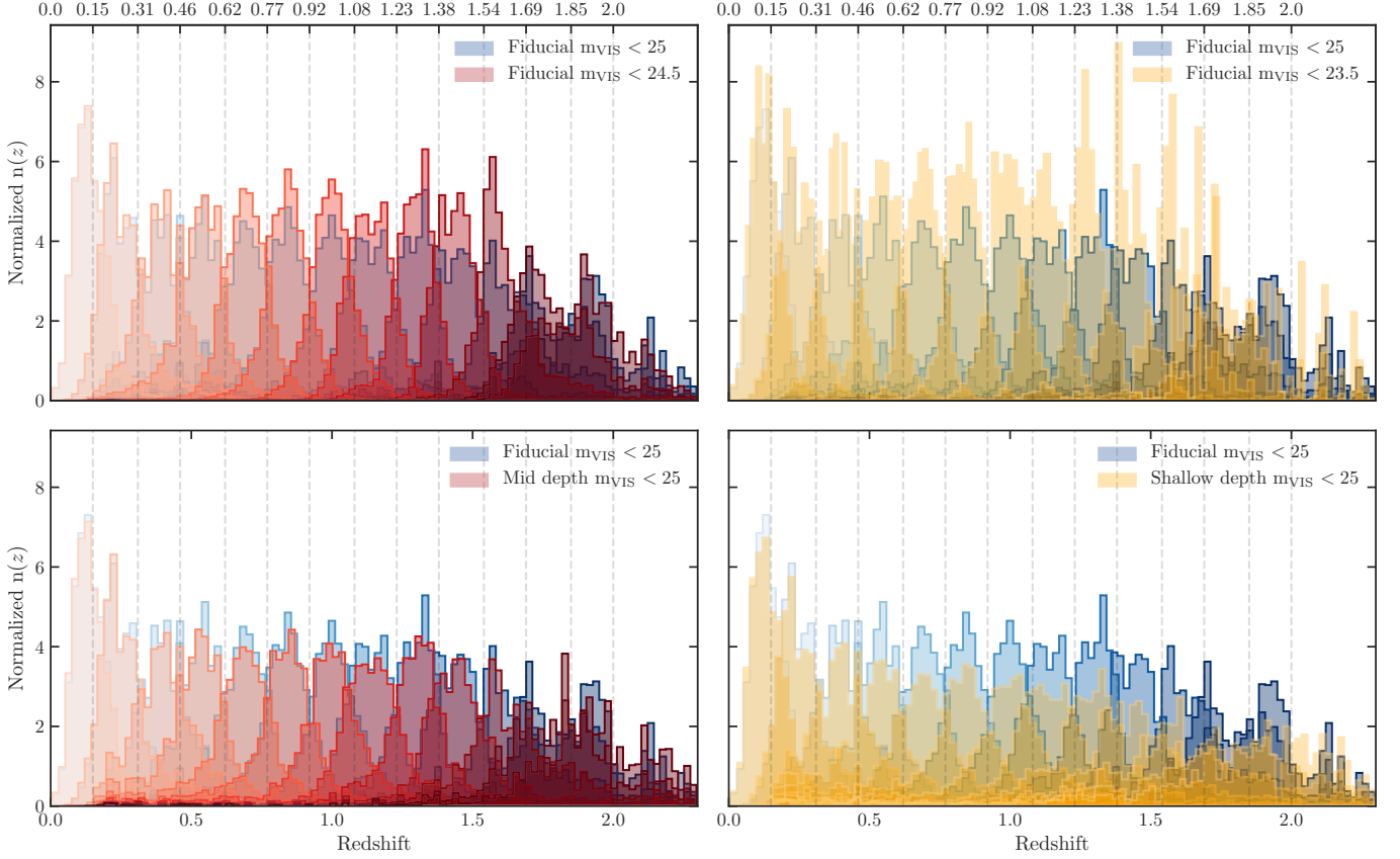
Fig. 14. Top panels: redshift distribution ( z_{\text{mc}} ) of each tomographic bin for the fiducial sample at m_{\text{VIS}} < 25 compared to the fiducial at m_{\text{VIS}} < 24.5 (left) and 23.5 (right). Bottom panels: redshift distribution ( z_{\text{mc}} ) of each redshift bin for the fiducial sample compared to the mid depth (left) and shallow depth samples at m_{\text{VIS}} < 25 (right).
