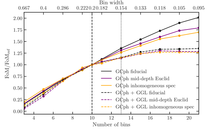
Fig. 7. FoM as a function of the number of bins with an equal width for GC ph (solid) and GC ph + GGL (dashed) for the mid depth Euclid and the inhomogeneous spectroscopic sample in addition to the fiducial sample, as in Fig. 6.
