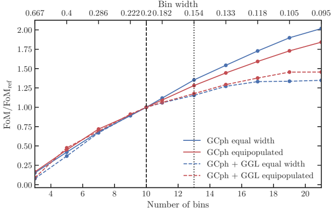
Fig. 6. FoM as a function of the number of bins for GC ph (solid) and GC ph + GGL (dashed), and for bins with the same redshift width (blue) and with the same number of objects (red). The redshift width of the bins when they have the same width is shown in the top x axis. The FoMs are normalized to the FoM at ten bins, FoM ref , which corresponds to the specifications for the number of bins used to compute the forecasts in EC20 and denoted by a vertical-dashed line. A vertical-dotted line shows the 13 bins used as our fiducial choice.
