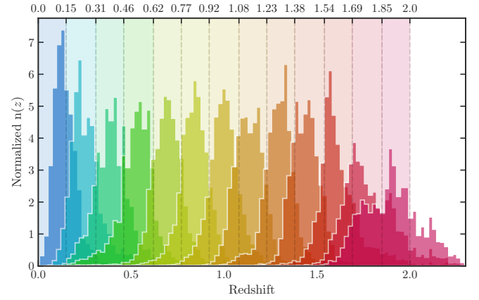
Fig. 8. Redshift distributions ( z_{\text{mc}} ) of the 13 bins with an equal width for the fiducial sample (case 2). The top x -axis correspond to the values of the redshift limits of the 13 bins with an equal width in redshift. The shaded regions indicate these limits.
