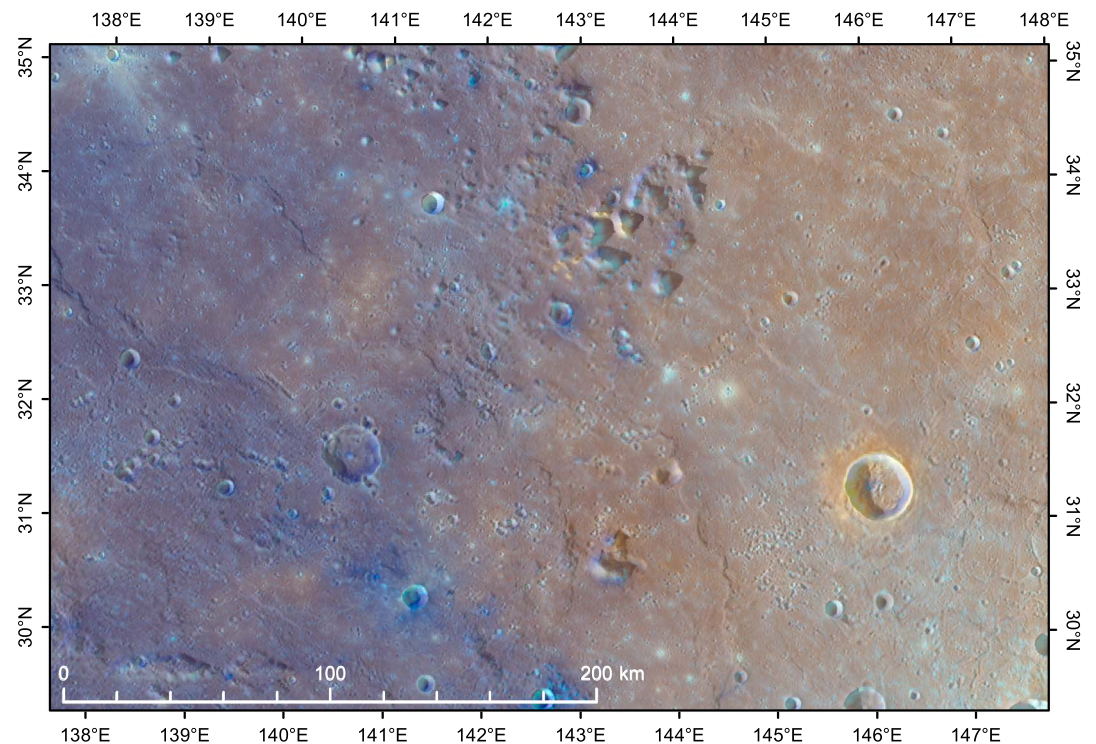
Figure 5. Location 4, with 665 mpp WAC color overlay on 166 mpp NAC mosaic. Note the diffuse and patchy gradual color transition between exterior plains (on the left) and interior plains (on the right).
