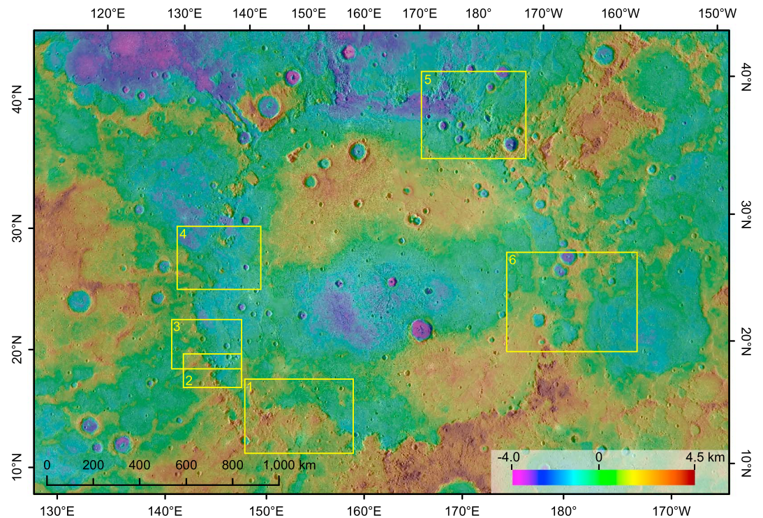
Figure 2. Color-coded topography of the Caloris basin.
