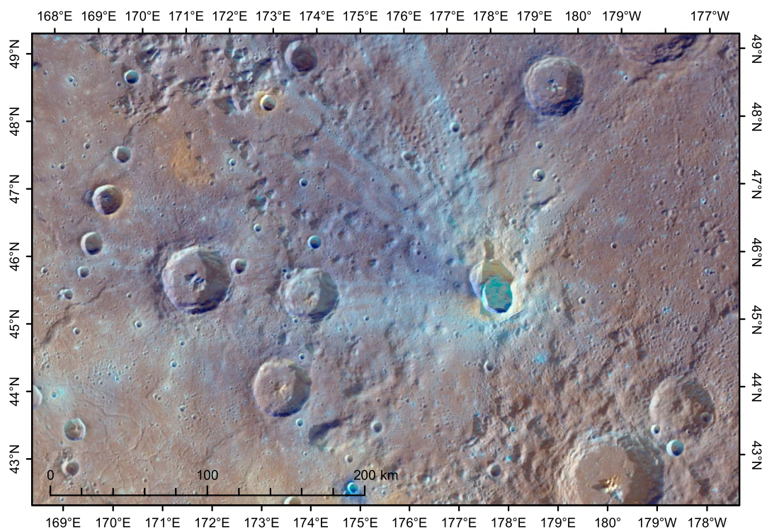
Figure 15. Location 5, with 665 mpp WAC color overlay on 166 mpp NAC mosaic. The rayed crater at 178°E is Ailey.
