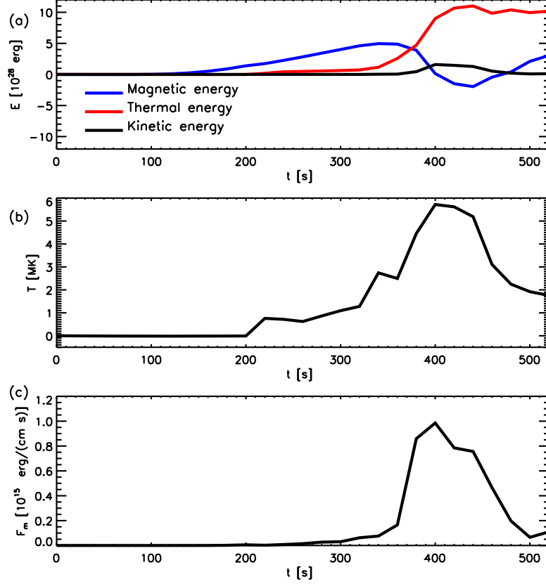
Supplementary Figure 10: Evolution of energies and temperature in the reconnection region (relative to initial values) . The magnetic, thermal and kinetic energies (panels a) are integrated in a volume near the centre of the domain that contains the region where the jet develops. The volume extends in the x -direction from x = -0.64 Mm to x = +0.64 Mm, in y -direction from y = -4 Mm to y = 0 Mm, and in z -direction from z = -2.6 Mm to z = +2.6 Mm and quantities are shown with respect to their value at t = 0 s. The temperature (panel b) corresponds to the maximum temperature in the same volume. The electromagnetic energy inflow rate into the reconnection region (panel c) corresponds to Eq. 4.
