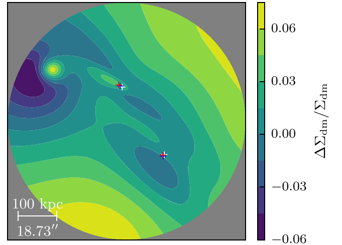
Figure 8. Relative difference between the proposed method and an a posteriori analysis in the diffuse dark matter surface mass density. Plus signs mark the BCGs (white) and the peaks of the diffuse dark matter distribution of the GAS (red) and POST (blue) models, respectively.
