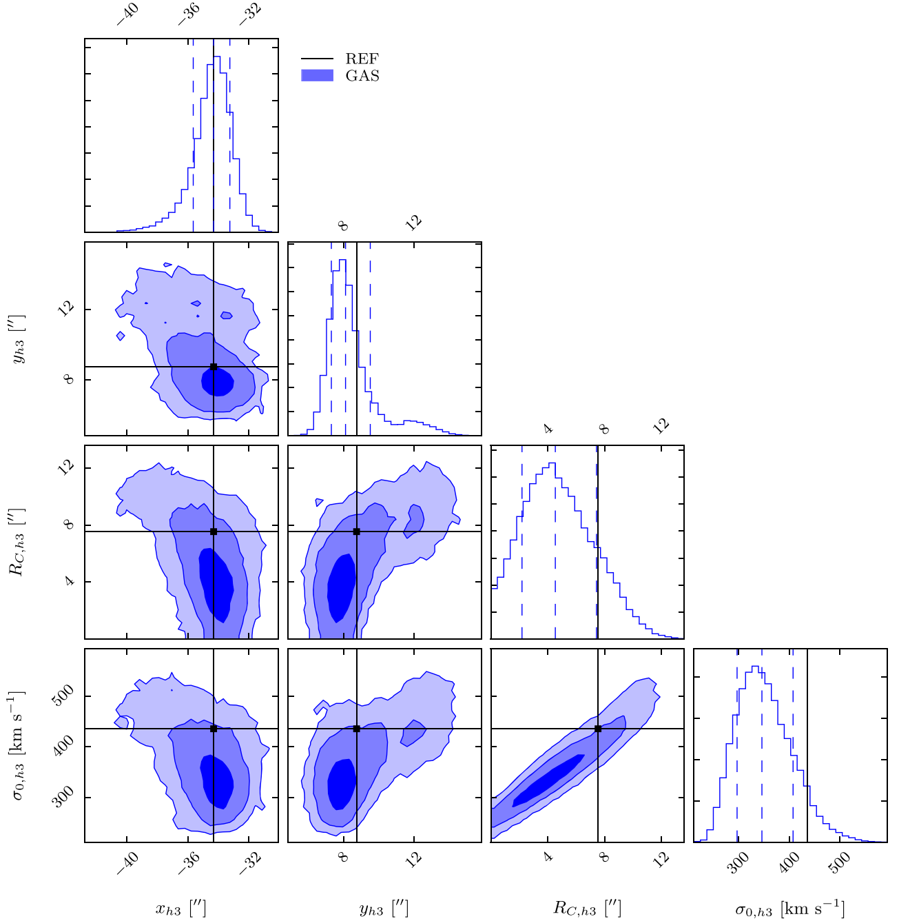
Figure 11. Posterior distributions of the values of the third main halo parameters derived from the strong-lensing model with the hot gas included separately (i.e., GAS model). Blue contours contain 39.3%, 86.5%, and 98.9% of the samples, while blue dashed lines in the 1D histograms show the 16th, 50th, and 84th percentiles. Black solid lines mark the median values of the reference model (i.e., REF model).
