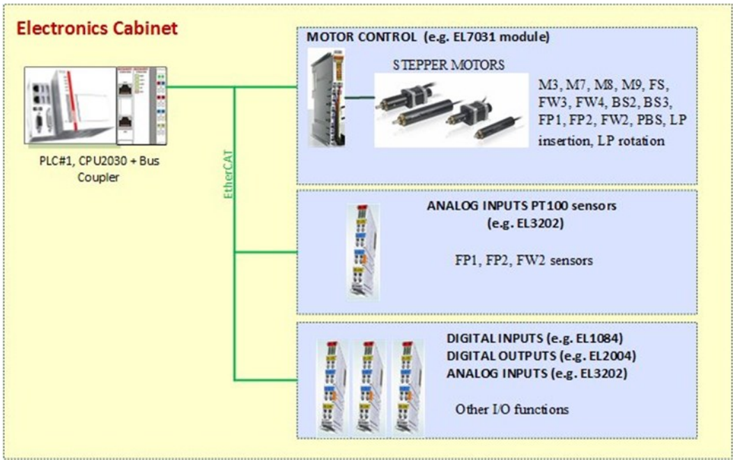
Figure 35: Beckhoff control architecture overview.
