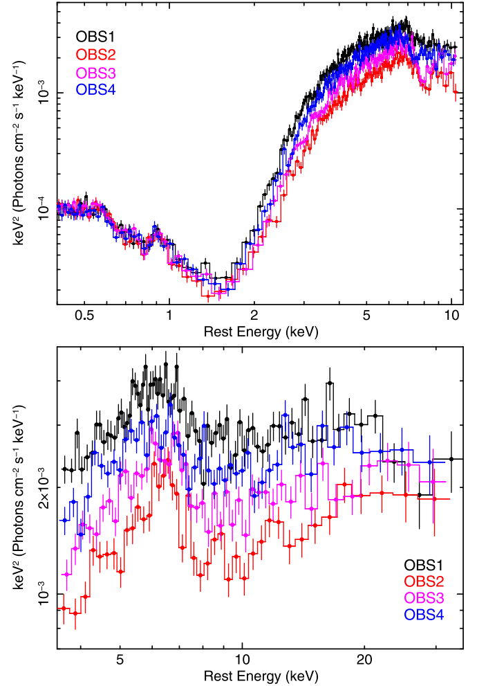
Figure 3. Upper panel: broadband (rest frame 0.4–10.5 keV) XMM-Newton spectra of the four observations of MCG-03-58-007 performed in 2019. The EF_E spectra are obtained unfolding the data against a simple power-law model with \Gamma = 2 . No variability is present below 2 keV, where the emission is dominated by the scattered component, while clear variability is present at higher energies, where MCG-03-58-007 dropped in flux during the OBS2. During OBS3, MCG-03-58-007 was in a slightly brighter state, but with an absorption structure almost as deep as in OBS2. Lower panel: NuSTAR spectra of the same observations. Like for the XMM-Newton data, the spectra are plotted against a simple \Gamma = 2 power-law model. The NuSTAR data independently confirms the presence of the deep absorption structures.
