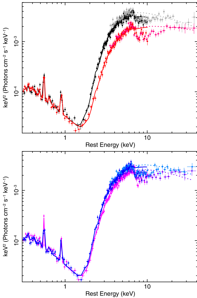
Figure 5. Broadband (rest-frame) pn and FPM spectra unfolded against the baseline continuum model described in Section 4.2. Upper panel: OBS1 (pn and FPM are shown in black squares and gray filled circles, respectively) and OBS2 (pn and FPM are shown in red squares and dark red filled circles, respectively). Lower panel: OBS3 (magenta squares and purple filled circles) and OBS4 (blue squares and light blue filled circles). Here the baseline continuum model is able to account for the overall spectral shape of the X-ray emission of MCG-03-58-007.
