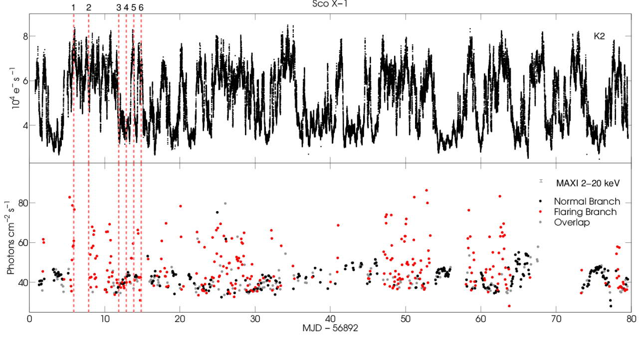
Figure 2. Top panel: K2 Sco X-1 light curve. The system was observed for over 78 days at 58.8 second cadence. The units on the y-axis are electrons/second, and can be converted to Kepler magnitudes K_p using the conversion found in the Kepler Instrument Handbook. Bottom panel: 2-20 keV MAXI light curve during the same period. Data points are colour coded using the NB/FB decomposition shown in Fig. 7. Typical MAXI error bar is shown on the top-right. The vertical dashed lines mark the times of our HERMES observations.
