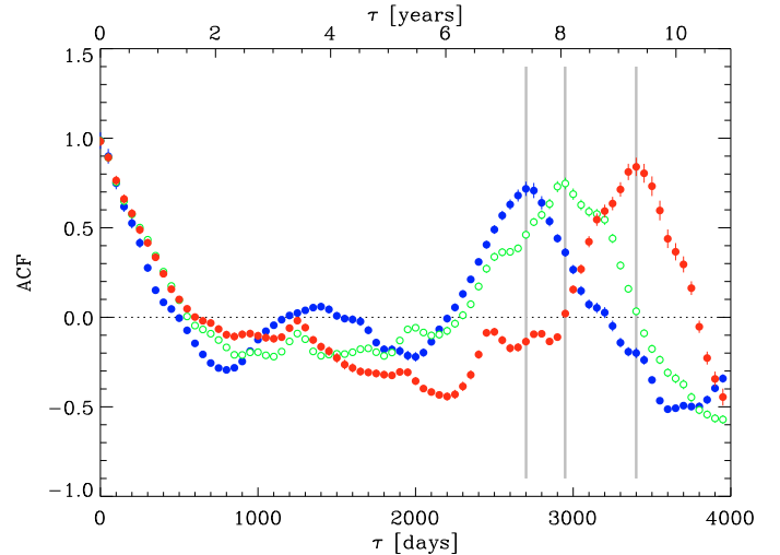
Fig. 3. Auto-correlation functions on subsequent pairs of radio outbursts at 8 GHz. Blue filled circles refer to the period JD = 2443 000–2449 000, green empty circles to JD = 2446 000–2452 000, and red filled circles to JD = 2449 000–2453 700.
