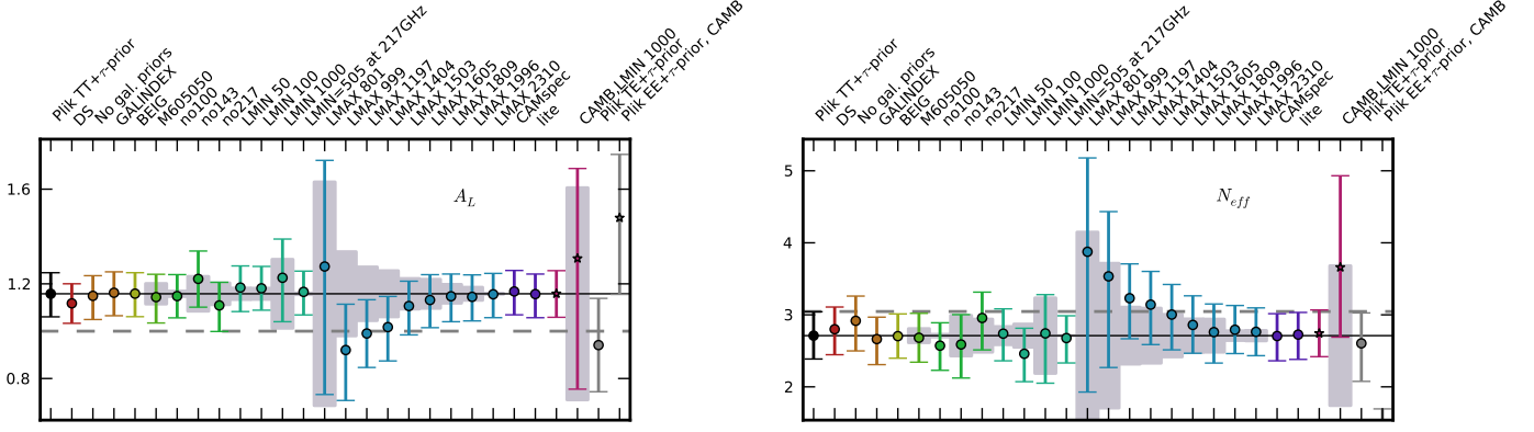
Figure 36. Marginal mean and 68 % CL error bars on the parameters A_L (left) and N_{\text{eff}} (right) in \Lambda CDM extensions, estimated with different data choices for the PlikTT likelihood in comparison with results from alternate approaches or model, combined with a Gaussian prior on \tau = 0.07 \pm 0.02 (i.e., neither low- \ell temperature nor polarization data). The “PlikTT+tauprior” case indicates the baseline (HM, \ell_{\text{min}} = 30 , \ell_{\text{max}} = 2508 ), while the other cases are described in subsections of Sect. 4.1. The thin horizontal black line shows the baseline result and the thick dashed grey line displays the \Lambda CDM value ( A_L = 1 and N_{\text{eff}} = 3.04 ). The grey bands show the standard deviation of the expected parameter shift, for those cases where the data used is a sub-sample of the baseline likelihood (see Eq. 53).
