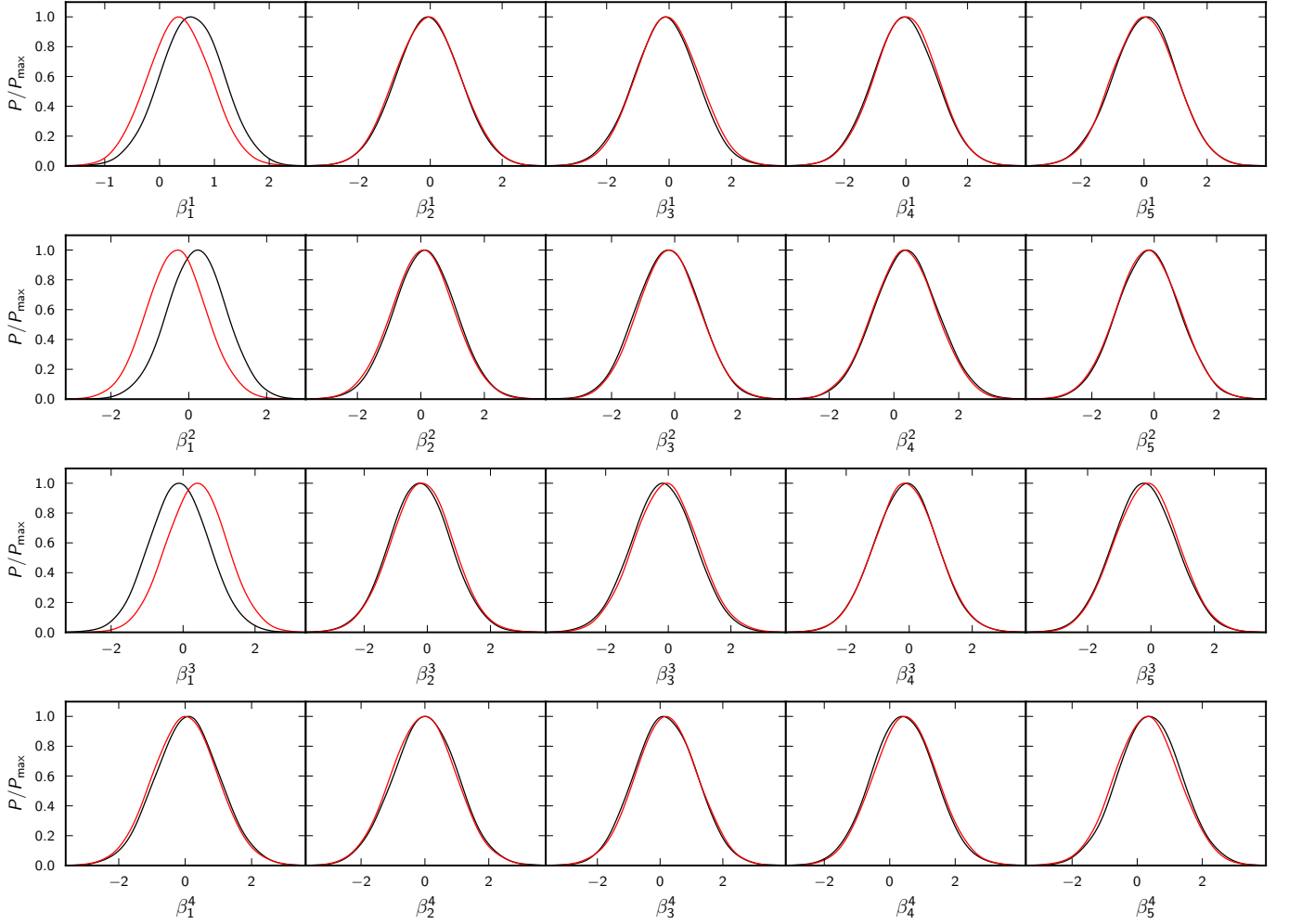
Fig. 17. Changes in the beam eigenmode coefficients from the inclusion of the near-sidelobe power now established but not included in the processing for the 2013 results. Black curves are for Planck +WP; red curves are for Planck +WP with the revised beams. The superscript indicates the effective spectrum (one to four for 100, 143, 217, and 143 \times 217 respectively) while the subscript indicates eigenmode number.
