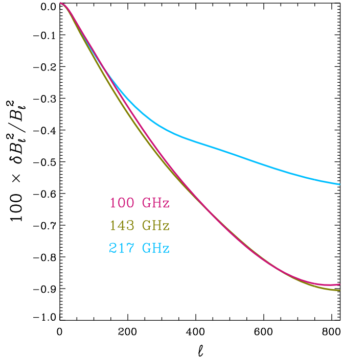
Fig. 11. Effective beam window function corrections from Fig. C.3, which correct for the effect of near-sidelobe power missing in the HFI beams used in the 2013 results (Sect. C.2.1). Uncertainties are not shown here for clarity, but are shown in Fig. C.3, and would be large on the scale of this plot. The 217 GHz correction is shown for illustration only.
