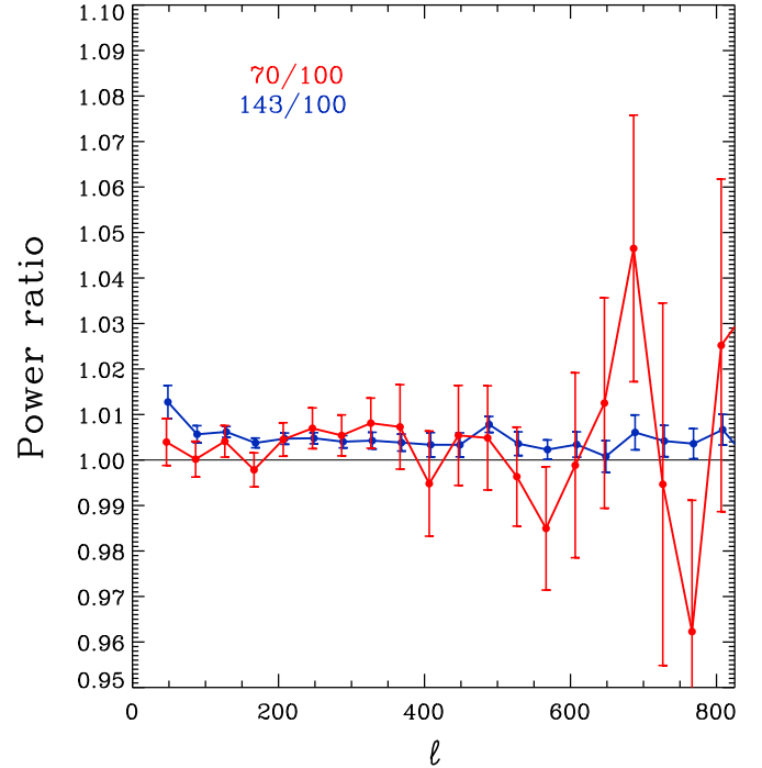
Fig. 13. Same as the bottom middle panel of Fig. 6, but corrected for both the near-sidelobe power at 100 and 143 GHz that was not included in the 2013 results and for unresolved source residuals (Sect. 3.3). Uncertainties in the beam window function corrections are not included.
