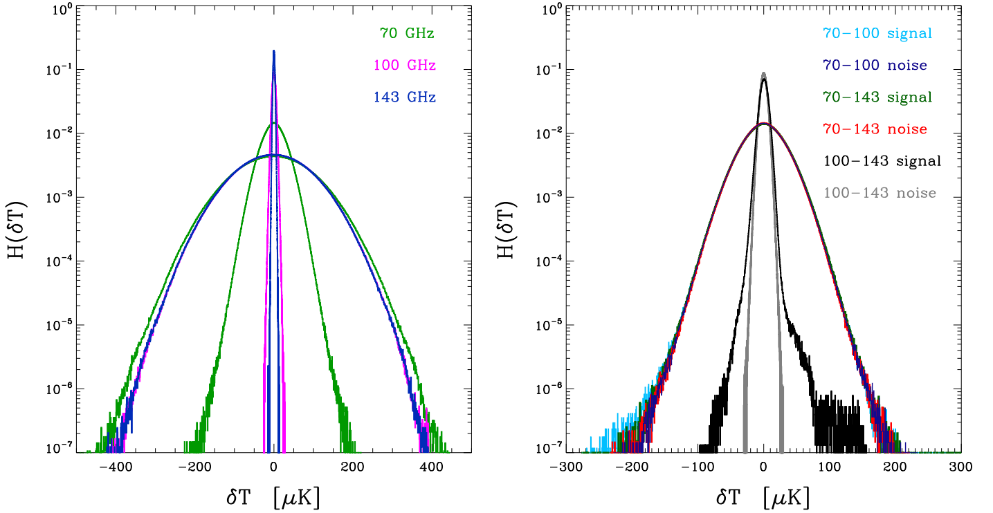
Fig. 4. Signal and noise for the frequency maps of Fig. 2 (left panel) and the difference maps of Fig. 3 (right panel), with the 59.6 % mask in all cases. The broader, signal+noise curves are nearly Gaussian due to the dominant CMB anisotropies. The 70 GHz curve is broader than the 100 and 143 GHz curves because of the higher noise level, but is still signal-dominated for |dT/T| \gtrsim 50 \mu\text{K} . The narrower noise curves, derived from the half-ring difference maps, are not Gaussian because of the scanning-induced spatial dependence of pixel noise in Planck maps. The considerably higher noise level of the 70 GHz map is again apparent. The histograms of the difference maps show noise domination near the peak of each pair of curves (the signal+noise and noise curves overlap). The pairs involving 70 GHz are wider and dominated by the 70 GHz noise, but the wings at low pixel counts show the signature of foregrounds that exceed the noise levels, primarily dust and CO emission in the negative wing, and free-free and synchrotron emission in the positive wing. In the low-noise 100 minus 143 GHz pairs, the signal, due mostly to dust emission in the negative wing and to free-free and CO residuals in the positive wing, stands out clearly from the noise.
