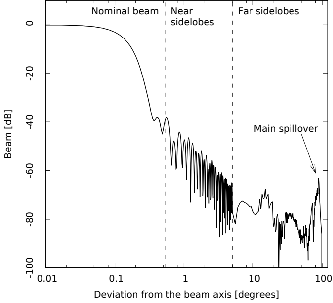
Fig. 10. Radial slice through a 70 GHz beam from the GRASP model, illustrating the nominal beam, near sidelobe, and far sidelobe regions. The exact choice of angular cutoff for the nominal beam is different for different frequencies.
