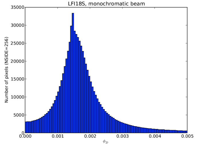
Fig. C.1. \phi_{\text{D}} for a simulation using a 70 GHz beam.
