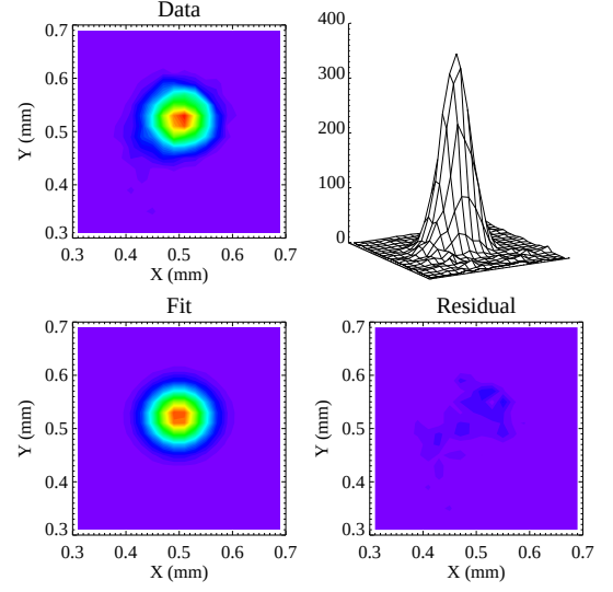
Figure 15: Image of a narrow X-ray beam detected by the GPD and fitting with a 2D Gaussian profile. The beam size is around 30 \mu\text{m} in FWHM and the intrinsic point spread function is measured to have a FWHM of about 78 \mu\text{m} .
