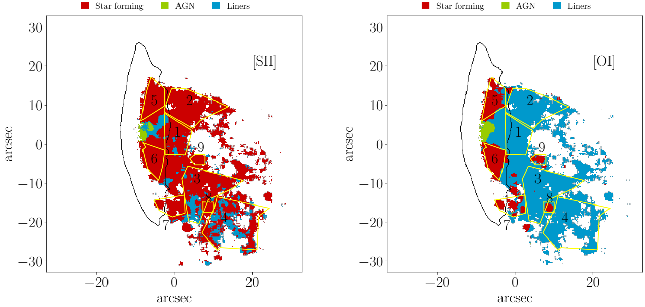
Figure 2. Ionization mechanism map according to (left) the [OIII]5007/H \beta vs [SII]6717,6731/H \alpha and (right) the [OIII]5007/H \beta vs [OI]6300/H \alpha diagnostic diagrams. Red=star formation. Green=AGN. Blue= LINER-like emission. The yellow polygons define the regions that are studied in §5.3. The black contour shows the stellar disk as in Fig. 1.
