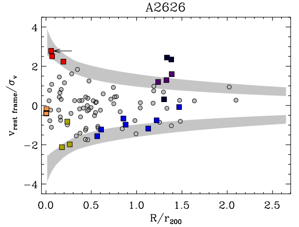
Figure 3. Distribution of cluster members in projected phase-space. Projected clustercentric distances R and rest-frame line-of-sight velocities v_{rf} are in units of the cluster virial radius and velocity dispersion, respectively (both taken from Biviano et al. 2017). Galaxies belonging to different substructures are represented by colored squares, each color defining a different substructure. The star symbol identifies JW100, which belongs to the substructure that includes also the two galaxies identified by the red squares. The grey-shaded regions represent the escape velocity curves with 1\sigma uncertainties, assuming a Navarro et al. (1996) profile and Tiret et al. (2007) velocity anisotropy profile. The width of these regions take into account 1\sigma uncertainties in the mass profile parameters r_{200} and r_{-2} from Biviano et al. (2017), and allowing the Tiret et al. (2007) profile parameter \beta_{\infty} (see eq.8 in Biviano et al. (2013)) to vary from 0 (isotropic orbits) to 0.75 (radial orbits).
