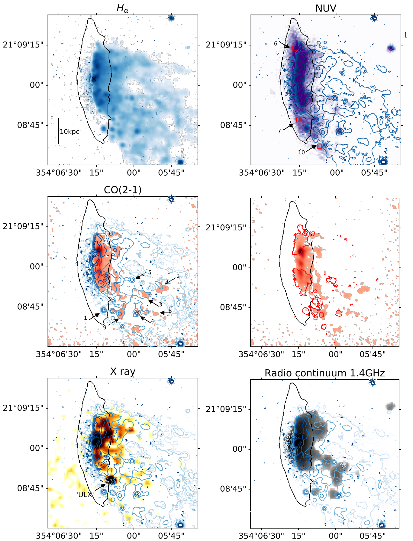
Figure 7. JW100 multi-wavelength tails. Images displayed are the MUSE H\alpha ( 1'' resolution) and the UVIT NUV ( 1.2'' ) (top panels), ALMA CO(2-1) ( 1'' ) (middle), Chandra X-ray ( 0.5'' ) and VLA 1.4 GHz ( 3.8'' \times 3.4'' ) (bottom). Overlaid blue contours are the MUSE H\alpha emission. The red contours in the middle right panel outline the star-forming regions in Fig. 2. The stellar disk region is shown by the black contours. The positions marked with arrows and numbers are discussed in the text (§4.1). The cross in the top left panel identifies the galaxy center, defined as the centroid of the continuum (stellar) emission underlying the H\alpha line from MUSE.
