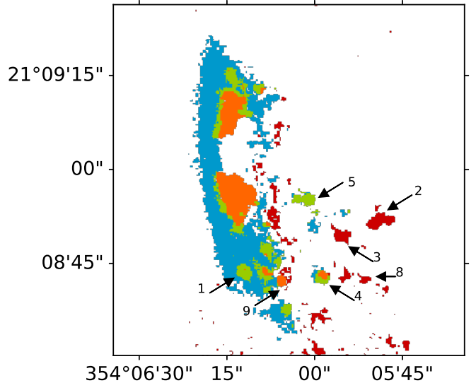
Figure 8. The star formation sequence created by ram pressure: only CO (red), CO+SF-powered H \alpha +UV (orange), SF-powered H \alpha + UV (green), and only UV (cyan). The regions with SF-powered H \alpha are star-forming also according to the [OI] line (right panel in Fig. 2). Numbers as in the middle left panel of Fig. 6.
