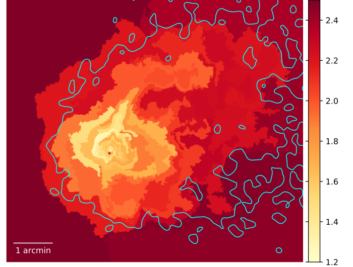
Figure 5. Photon index map of J1709. Spectral bins were defined following surface brightness contours. To the spectrum extracted from each bin, we fit a PL model with N_H set to 5 \times 10^{21} \text{ cm}^{-2} . The typical 90% error is 0.11. The edge of the wind bubble (see Figure 3) is shown as the cyan contour.
