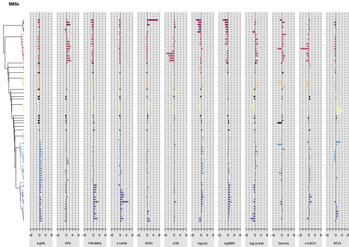
FIGURE 2 | Cladograms for the M85 sample rooted with the lowest- M_{\text{BH}} group, showing barplots for the Eddington ratio L/L_{\text{Edd}} in addition to the eleven parameters used to find the tree. Colors correspond to the groups defined from the tree on the left.
