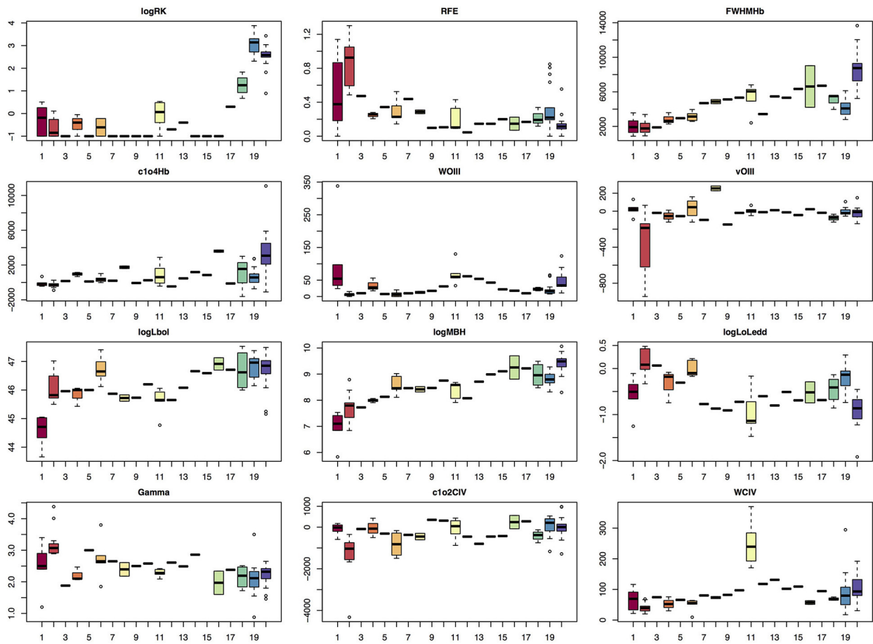
FIGURE 4 | Box plots with identified groups for the M85 sample. The ordinate axis shows the parameter coded on top of the plot, with code meaning explained in Section 2.3. Medians are thick horizontal lines while boxes define limits from first to third interquartile range. Outliers are shown as open circles. Colors correspond to those in Figure 2 .
