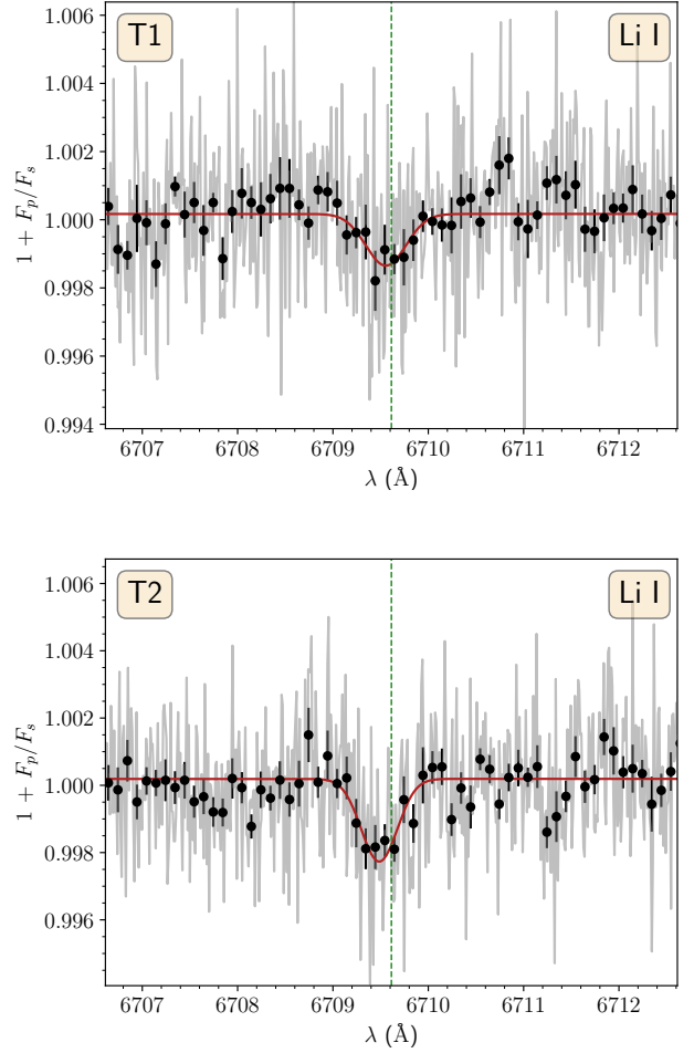
Fig. 10. Same as Fig. 6 but for the Li I line.
