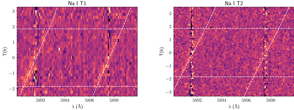
Fig. 5. Na Double tomography for transit 1 ( left ) and transit 2 ( right ). Time 0.0 h corresponds to the mid-transit according to the planetary ephemeris given in Table 3. Each tile represents a 0.1 Å bin. These plots are qualitative and have been generated only for visualisation purposes.
