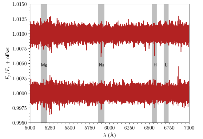
Fig. 3. Transmission spectra for WASP-76b in the 5000–7000 Å range: a few key features are shaded in grey. The T1 is the top spectrum and T2 is the bottom one. A binning of 0.1 Å has been applied to the data for clarity. All wavelengths are given in vacuum.
