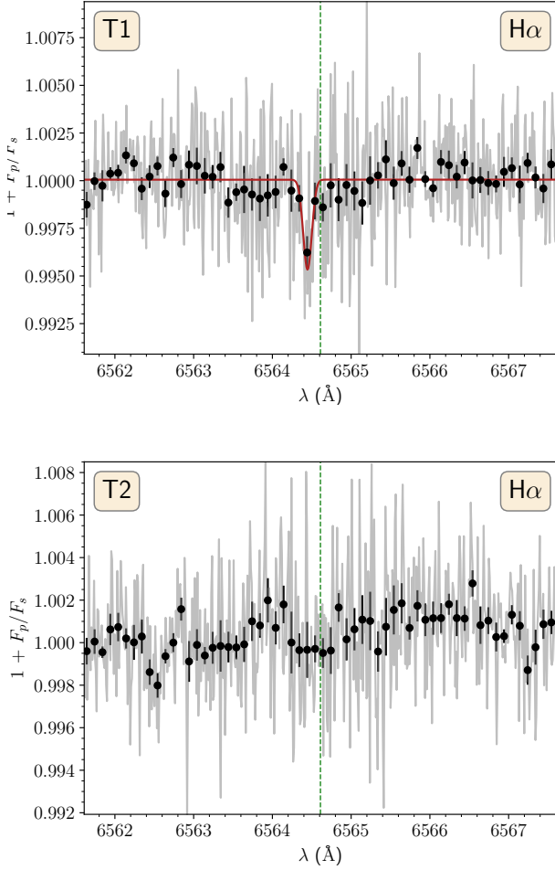
Fig. 9. Same as Fig. 6 but for the H\alpha line.
