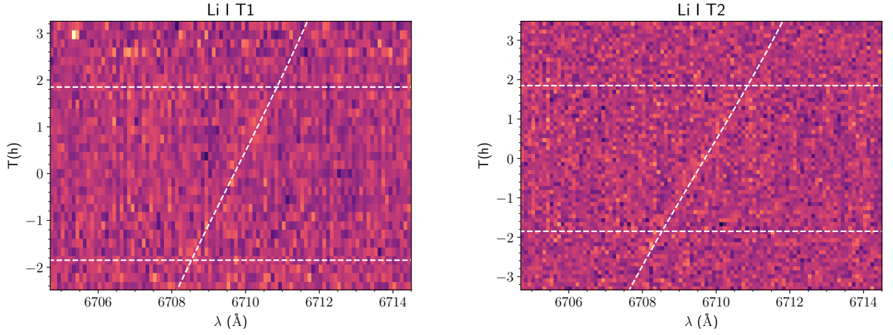
Fig. A.4. Same as Fig. 5 but for Li I.
