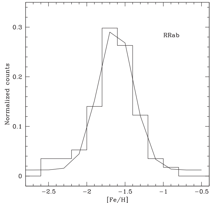
Figure 6. Metallicity distribution of And XXVII RRab stars obtained using Alcock et al.'s (2000) method. The distribution peaks at [\text{Fe}/\text{H}] \sim -1.62 , with \sigma \sim 0.23 dex.
