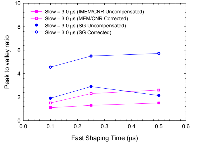
Fig. 14. Peak-to-valley ratio before and after compensation as a function of the fast shaping time at 662 keV.
