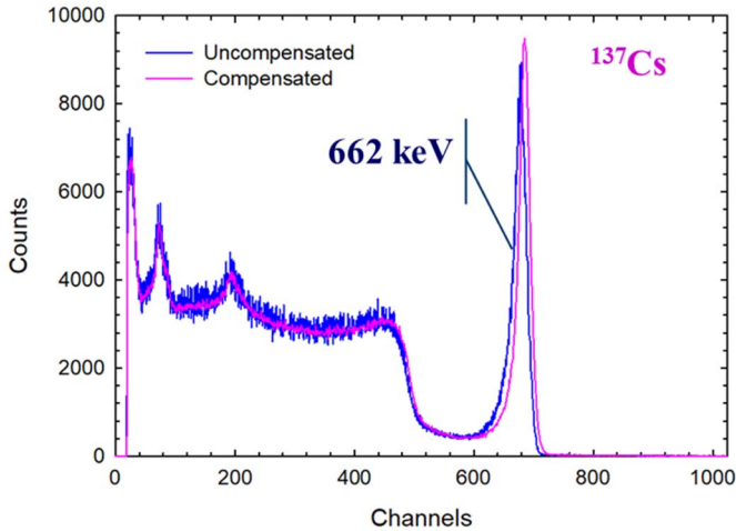
Fig. 16. ^{137}\text{Cs} spectra acquired with a 0.25–3.0 \mu s shaping time pair. The blue plot represents the original spectrum, while the pink one is the spectrum after compensation.
