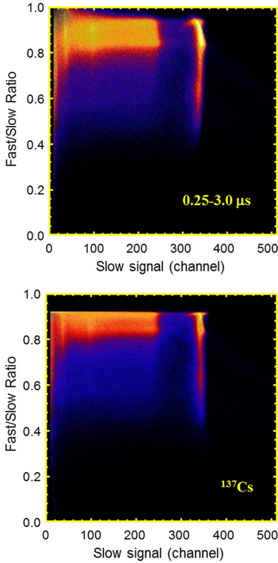
Fig. 15. Comparison of the uncompensated (top) and corrected (bottom) maps acquired with the drift strip detector provided by CNR/IMEM and a 0.25–3.0 \mu s shaping time pair.
