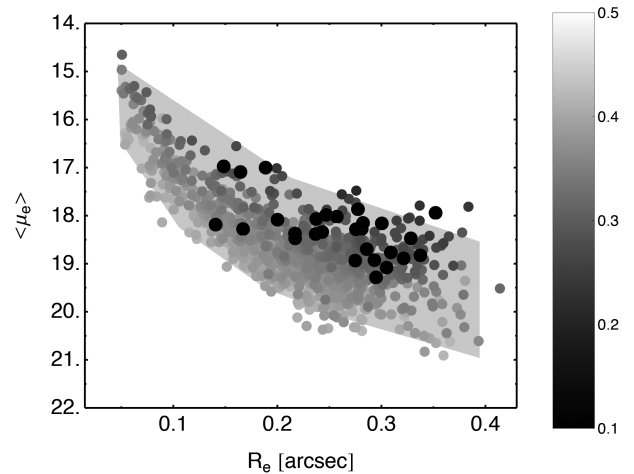
Figure 4. \langle\mu_e\rangle – R_e plane. Small dots are for the UCMG_PHOT sample using MFREE masses and with z_{\text{phot}} \leq 0.5 . The points are colour coded accordingly to their photometric redshift (a colour bar is added to the plot). Larger black dots with grey edges are for all the UCMG candidates in UCMG_NEW. Shaded grey region encloses the 2DPHOT \langle\mu_e\rangle and R_e output values for the mock galaxies simulated in Appendix B. The lower bound of the shaded region corresponds to galaxies with m_S \sim 21 , which is approximately our magnitude limit.
