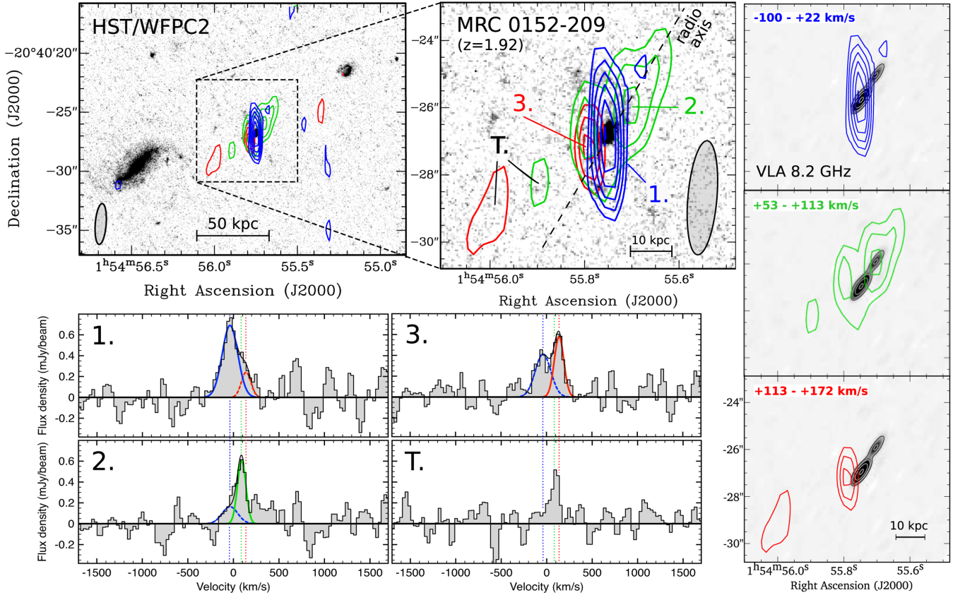
Figure 4. Top left: total intensity image of MRC 0152-209 integrated over three distinct velocity ranges (blue = -100 - +22 \text{ km s}^{-1} ; green = 53 - 113 \text{ km s}^{-1} ; red = 113 - 172 \text{ km s}^{-1} ) and overlaid on to the HST/WFPC2 image of Fig. 1 to within an accuracy of \lesssim 0.5 arcsec (part of this figure is reproduced, with permission, from Emonts et al. 2014, their Fig. 4). CO(1–0) contour levels are at 2.8\sigma , 3.5\sigma , 4.2\sigma , 4.9\sigma , 5.6\sigma , 6.3\sigma level (with \sigma = 12 \text{ mJy beam}^{-1} \times \text{km s}^{-1} for the blue component and 7.3 \text{ mJy beam}^{-1} \times \text{km s}^{-1} for the red/green components). The dashed line visualizes the extrapolated radio axis. Right: plots of the individual total intensity maps, as extracted across the three different velocity ranges. The 8.2 GHz radio continuum source from Pentericci et al. (2000) is overlaid in grey-scale and thin contours (levels at 2, 7, 25 and 86 per cent of the peak intensity). Bottom: CO(1–0) emission-line spectra in the four distinctive regions indicated in the total intensity plot on the top. The data are Hanning smoothed and the velocity is shown with respect to z = 1.9212 (Section 2). The solid blue, green and red lines represent Gaussian fits to the CO emission from regions 1, 2 and 3, respectively. From the flux covered by these Gaussians we derived L'_{\text{CO}} for each region. The dashed coloured lines indicate the estimated spill-over emission from adjacent regions that are separated by one beam-size or less (this emission is not included in the determination of L'_{\text{CO}} ). The thin black line is the overall fit.
