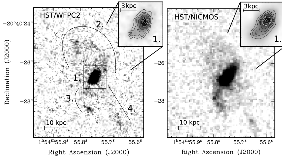
Figure 1. Left: HST /WFPC2 F555W image of MRC 0152-209. The four distinct features are described in the text. The inset on the top show a zoom-in of the central region #1. Right: HST /NICMOS F160W image at the same scale as the HST /WFPC2 image. The NICMOS data have been reproduced from Pentericci et al. (2001), their fig. 2. (© AAS; reproduced with permission.)
