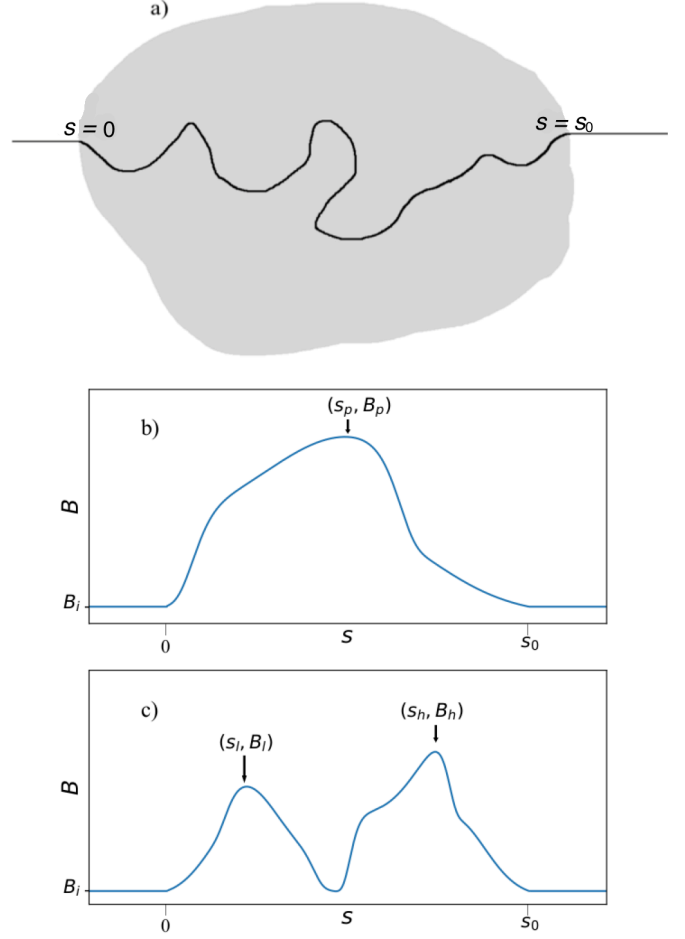
FIG. 1.— Panel (a) shows a sketch of a magnetic field line entering a cloud (grey region). Panels (b) and (c) depict sketches of the magnetic field strength B as a function of distance s along a field line. Panel (b) shows the single-peaked case discussed in Section 2.1, panel (c) shows the double-peaked case, Section 2.2.
