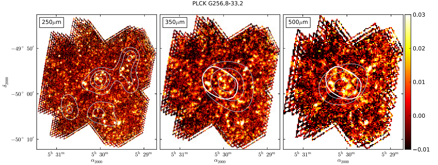
Fig. 1. SPIRE maps at 250, 350, and 500 \mu\text{m} of one typical overdensity in our sample (a Planck cold source of the CIB). The thick white contour at 350 \mu\text{m} shows the Planck IN region at 857 GHz, and the same is true for the map at 500 \mu\text{m} at 545 GHz (i.e., the 50% contour of the Planck source maximum). Thin contours correspond to the overdensity of SPIRE sources at each wavelength, marked at 2\sigma , 3\sigma , etc. (see Sect. 4.2 for details). SPIRE identifies a few (typically 5 to 10) sources inside the Planck contour. We use these contours to separate the IN and OUT zones. These data come from a 7' \times 7' SPIRE scan (see Table 1 and Sect. 2.3).
