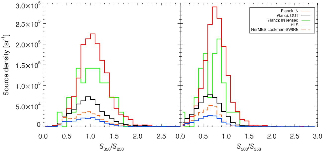
Fig. 7. Colour counts: source surface density as a function of the SPIRE colour, S_{350}/S_{250} (left), and S_{500}/S_{350} (right). Histograms are: red solid line, Planck IN; black line, Planck OUT; green, Planck IN lensed fields only; blue line, z < 1 HLS clusters; and orange dashes, Lockman SWIRE. The Planck IN sources (total and/or lensed sources) show a much higher surface density than other samples, owing mainly to our all-sky search strategy. See Sect. 4.3 for details.
