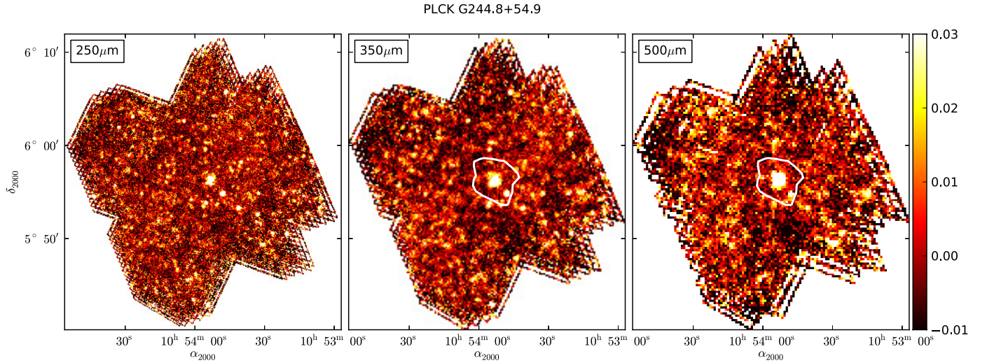
Fig. 2. SPIRE maps at 250, 350, and 500 \mu\text{m} for a lensed source. In this case a single very bright SPIRE source is detected. This source is confirmed at the Jy level and has a redshift of z = 3.0 , measured from multi-line spectroscopy acquired at IRAM using EMIR (Canameras et al., in prep.). The white contour is the Planck IN region, defined in the same way as in Fig. 1. These data come from a 7' \times 7' SPIRE scan (see Table 1 and Sect. 2.3).
