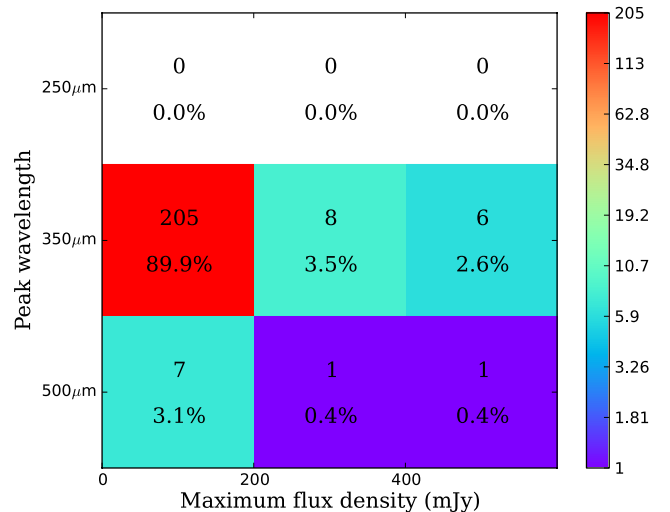
Fig. 9. Classification of 228 Planck fields with Herschel -SPIRE. The x -axis represents the maximum flux of the SPIRE source within the IN region: lensed source candidates are selected if they fall above 400 mJy (i.e., the right column, seven sources). The y -axis represents the wavelength at which the brightest SPIRE source peaks in the IN region. Overdensities are thus selected in the lower left four cells. The colour represents the number of fields in each cell (as shown in the colour bar), the numbers in the cells are the number of fields and percentage in each cell. Our sample is thus dominated by overdensities peaking at 350\,\mu\text{m} . See Sect. 4.4 for details.
