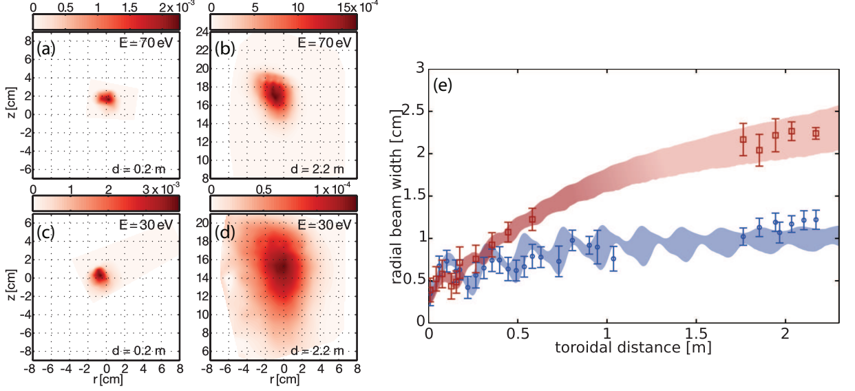
FIGURE 1. Left: poloidal suprathermal ion current profiles (units in A/m^2 ) at different toroidal distances for two ion energies (a, b) E = 70 eV, (c, d) E = 30 eV. The vertical drift due to the curvature and gradient of the magnetic field is shown. The spreading due to the interaction with the turbulent plasmas is more important for 30 eV ions. Right: radial width of suprathermal ion current profiles as a function of toroidal distance. Red squares and blue circles represent experimental measurements for ions emitted at 30 eV and 70 eV respectively. Continuous bands are obtained from a synthetic diagnostic using numerical simulations for 30 eV (red) and 70 eV (blue) ions. The width of the bands is obtained by varying the simulations input parameters within experimental uncertainties. The different beam spreadings as a function of the toroidal distance indicate different transport regimes.
