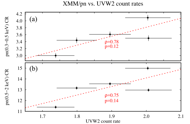
Figure 3. XMM-Newton /pn count rate, averaged over each observation, in the 0.3–0.5 keV band (panel A) and in the 0.5–2 keV band (panel B) plotted against the OM/UVW2 count rate. The red dashed lines represent linear fits to the data.
