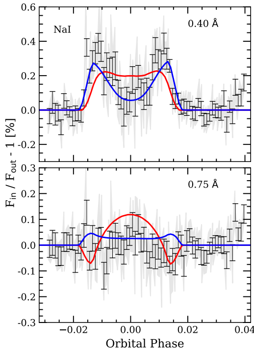
Fig. 6: Transmission light curves calculated in Na I doublet after combining both nights, using a 0.4 Å ( top ) and 0.75 Å ( bottom ) passbands. In light-grey, we show the original data. In black, we show the data binned by 0.001 in orbital phase. In red we show the impact of the CLV and RM effects in the transmission light curve. In blue, only the RM effect is considered.
