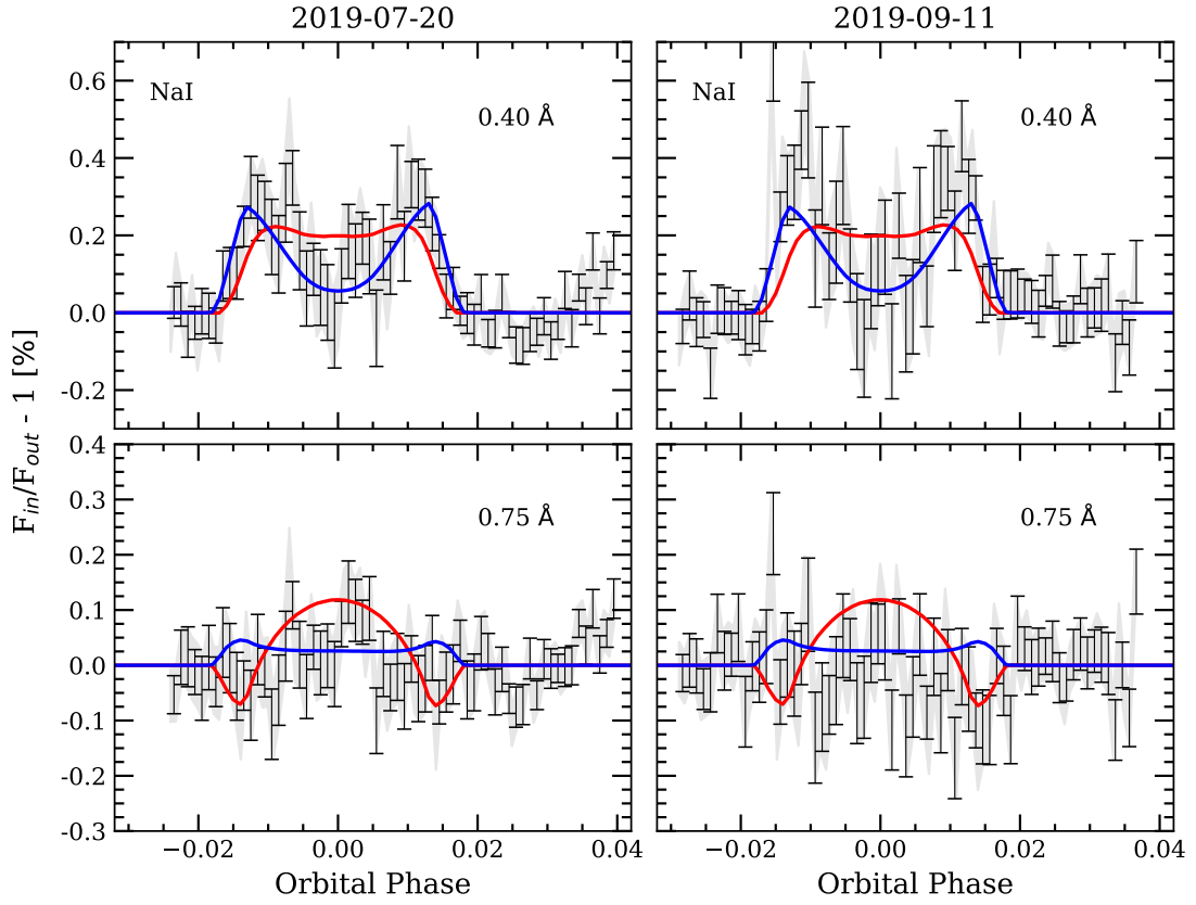
Fig. A.2: Same as in Figure 6, but for the individual nights: first night (2019-07-20) in the left column and second night (2019-09-11) in the right column. We note that the second night results could be partially affected by telluric Na I absorption residuals.
