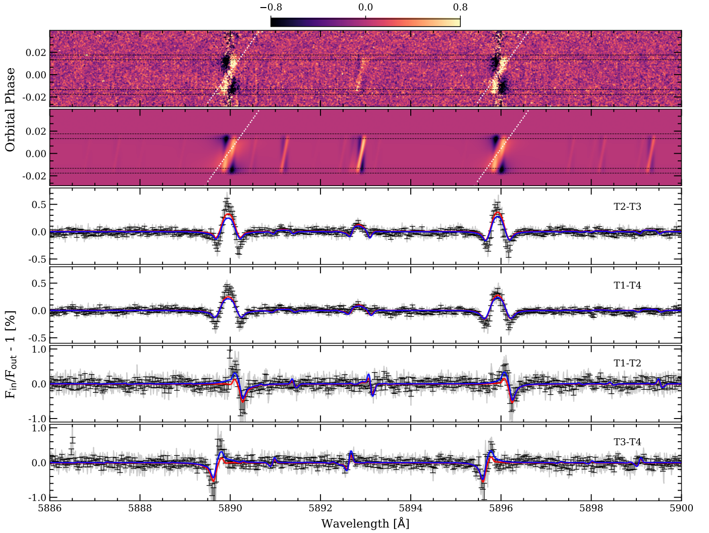
Fig. 5: First panel (top) : Two-dimensional map of the individual transmission spectra around the Na I doublet lines of HD 209458b. Second panel : Two-dimensional map of the modelled CLV and RM effects around the Na I doublet. In both panels, the results are presented in the stellar rest frame and the colour bar shows the relative flux ( F_{\text{in}}/F_{\text{out}}-1 ) in %. The black horizontal dashed lines indicate the four contacts of the transit and the dotted white line marks the expected position of the planet trail during the observations. Third panel : Transmission spectrum computed combining the data between the second and third contacts of the transit. Fourth panel : Combination of the in-transit exposures from the first to fourth contacts. Fifth panel : Combination of ingress exposures. Sixth panel (bottom) : Combination of egress exposures. The transmission spectra are computed combining the data in the planet rest frame. The original data error bars are shown in light grey and the data binned by 0.03 \text{ \AA} is shown in black. We note the different y-scale in the different panels. In red, we show the CLV and RM effects in the final transmission spectrum and in blue, the deformation due to the RM alone.
