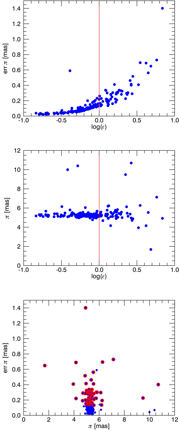
Fig. A.1. Upper two panels: distribution of the parallaxes and errors in parallax as a function of the astrometric excess noise. The vertical red line corresponds to the excess noise = 1. Bottom panel: parallaxes vs. the error in parallaxes. Sources excluded by our analysis are highlighted with red circles.
