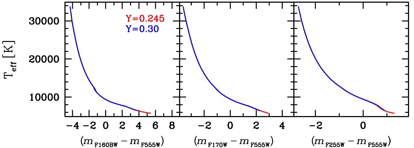
Figure 2. Same as Figure 1 but for the effect of the initial He mass fraction Y , for the three colors we will use in our study (see text for details).
