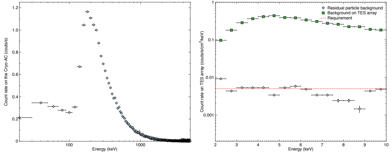
Figure 1. ( Left ) Count rate ( \text{cts s}^{-1} ) of the total Galactic Cosmic Background seen by the Cryo-AC over the 20 – 800 keV energy band simulated using GEANT-4 for \sim 900 s. The low-energy peak ( \sim 40 keV) is due to secondary particles, while primaries are responsible for the higher energy peak ( \sim 300 keV). ( Right ) Count rate ( \text{cts s}^{-1} \text{ cm}^{-2} \text{ keV}^{-1} ) seen by the entire TES array before (green squares) and after the CryoAC background reduction (blue diamonds). The red dashed line indicates the requirement of 5 \times 10^{-3} \text{ cts s}^{-1} \text{ cm}^{-2} \text{ keV}^{-1} .
