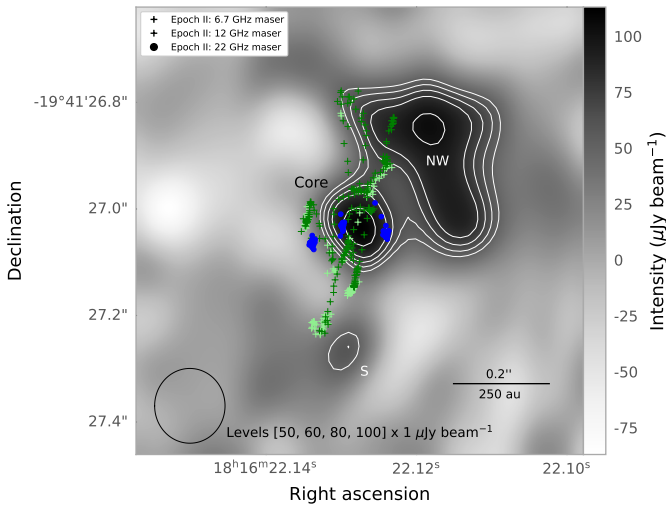
Fig. 4. 1.3 cm continuum image and masers detected at Epoch II towards CM1. Each continuum component of CM1 is labelled, and different types of masers are marked by colour (see the legend).
