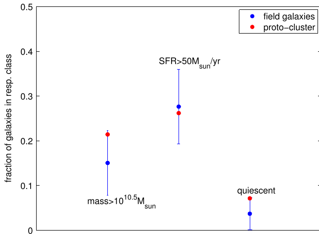
Figure 5. Fraction of massive M > 10^{10.5} M_{\odot} (left), highly star-forming \text{SFR} > 50 M_{\odot} \text{ yr}^{-1} (middle), and quiescent galaxies in the protocluster (red) and in the field (blue). There is a weak trend for more massive and quiescent galaxies within the protocluster; this is, however, not significant.
