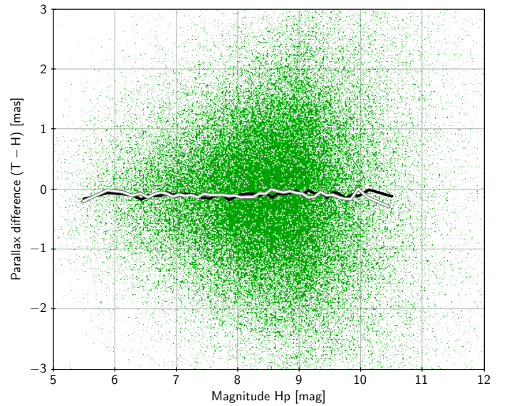
Fig. C.6. Parallax differences (TGAS minus HIPPARCOS) for 86 928 sources, plotted against magnitude. The black line is for northern ecliptic latitudes ( \beta > 0 ), the grey-white line for southern ( \beta < 0 ). The lines connect median values calculated in 50 bins subdividing the data according to the HIPPARCOS magnitude H_p . Each bin contains about 900 data points per hemisphere.
