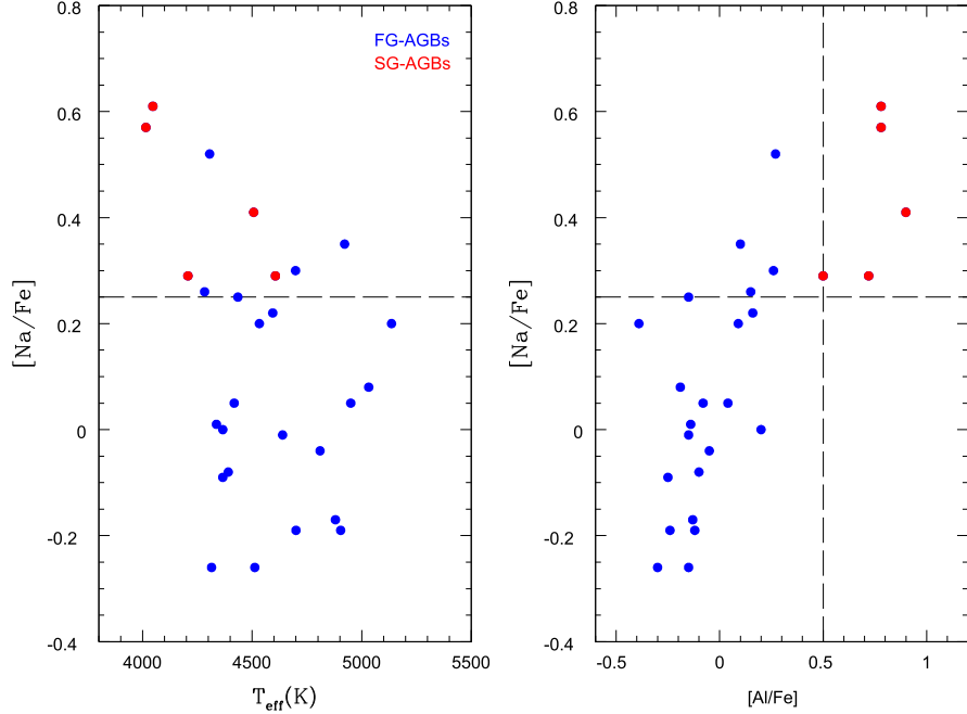
Figure 3. Literature [\text{Na}/\text{Fe}] abundances (corrected for NLTE) for our APOGEE sample of FG- and SG-AGB stars (blue and red dots, respectively) shown against stellar effective temperature T_{\text{eff}} (left panel) and Al abundances (right panel). The horizontal and vertical lines mark [\text{Na}/\text{Fe}] = +0.25 dex and [\text{Al}/\text{Fe}] = +0.50 dex, respectively and separate the FG-AGBs from the SG ones. The Na limit is set to [\text{Na}/\text{Fe}] = 0.25 dex, corresponding to the average upper limit for the [\text{Na}/\text{Fe}] value for FG field stars in the metallicity range covered by the GCs in our sample (see e.g., Carretta 2013).
