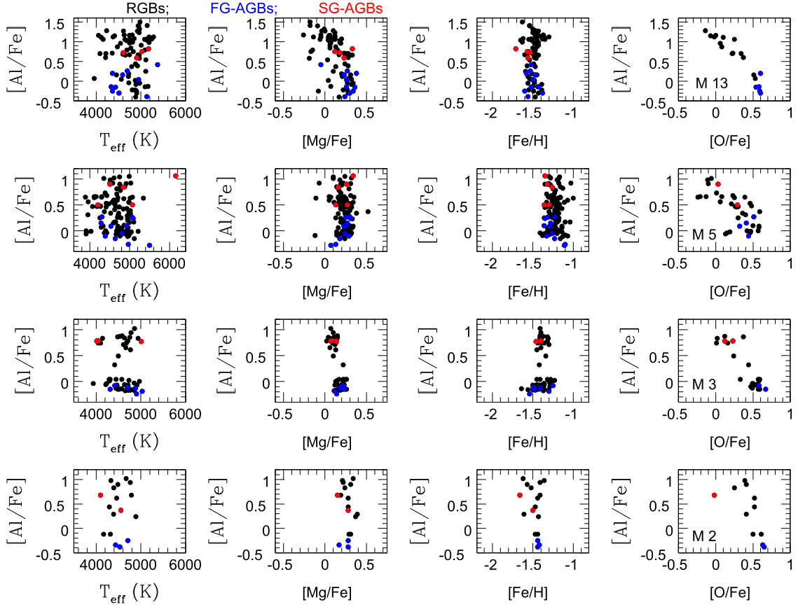
Figure 2. [\text{Al}/\text{Fe}] for our APOGEE sample of FG- and SG-AGB stars (blue and red dots, respectively) in metal-poor GC stars (from top to bottom: M13, M5, M3, and M2) shown against (from left to right) stellar effective temperature T_{\text{eff}} , [\text{Mg}/\text{Fe}] , [\text{Fe}/\text{H}] , and [\text{O}/\text{Fe}] . The APOGEE abundances are precise to the \sim 0.1 dex level. For comparison, the RGB stars (black dots) observed by APOGEE are also displayed. Note that the spread in [\text{Fe}/\text{H}] is bigger in RGB than in AGB stars because of the presence of warm stars, which lead to bigger uncertainties (consequently [\text{Al}/\text{Fe}] is determined with higher accuracy in AGB than in RGB stars).
