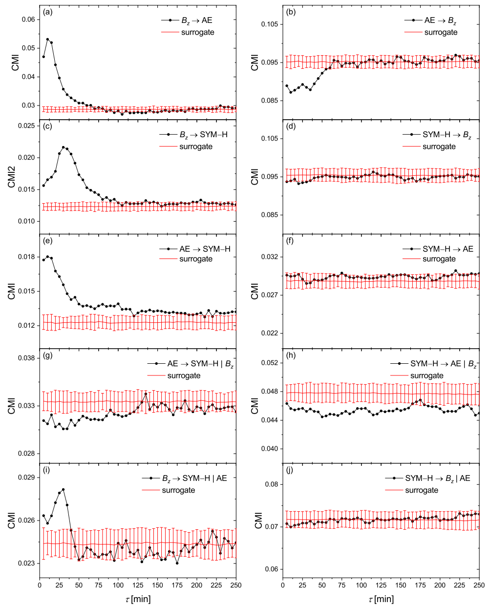
Figure 3. The conditional mutual information (CMI) (Equation (13)) obtained from the time series of B_z , AE and SYM-H, for the information flow directions of (a) B_z \rightarrow AE, (b) AE \rightarrow B_z , (c) B_z \rightarrow SYM-H, (d) SYM-H \rightarrow B_z , (e) AE \rightarrow SYM-H, and (f) SYM-H \rightarrow AE. (g,h) are the information flow directions similar to (e,f), by taking B_z as the third variable into the condition (see Equation (18)). Analogously, (i,j) are the information flow directions similar to (c,d), by taking AE as the third variable into the condition. The red lines and error bars present mean and \pm 2 standard deviations of CMI for a set of circular time-shifted surrogates.
