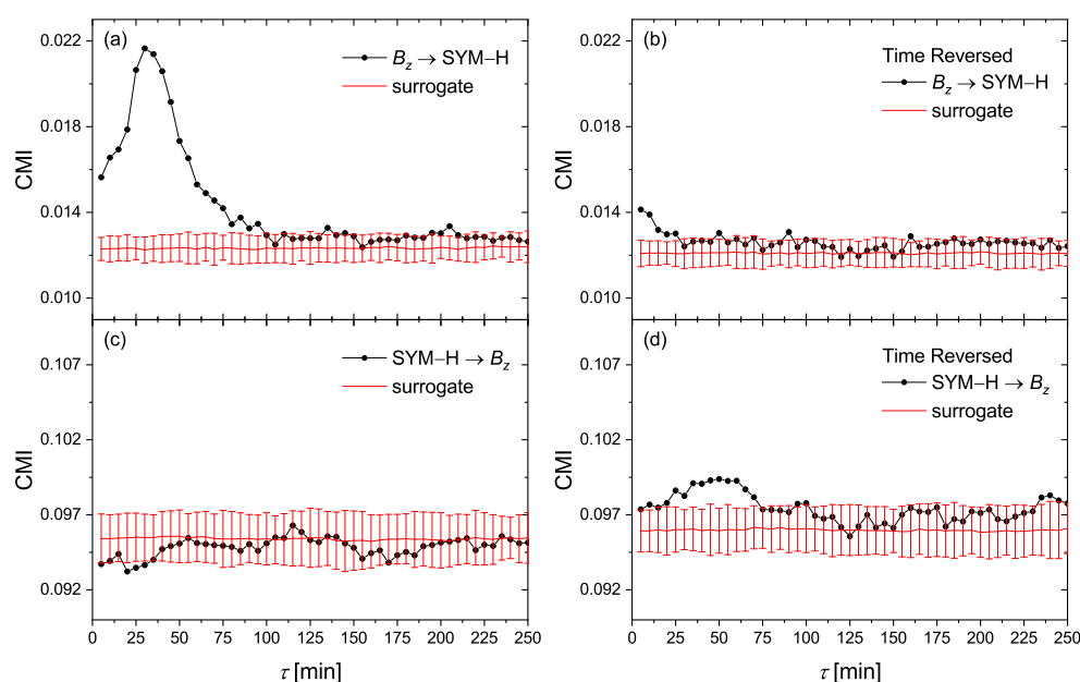
Figure 5. The conditional mutual information (CMI) of Equation (13) for the information flow directions of (a) B_z \rightarrow SYM-H , (c) SYM-H \rightarrow B_z . (b,d) are, respectively, the same as (a,c), but for time-reversed series.
