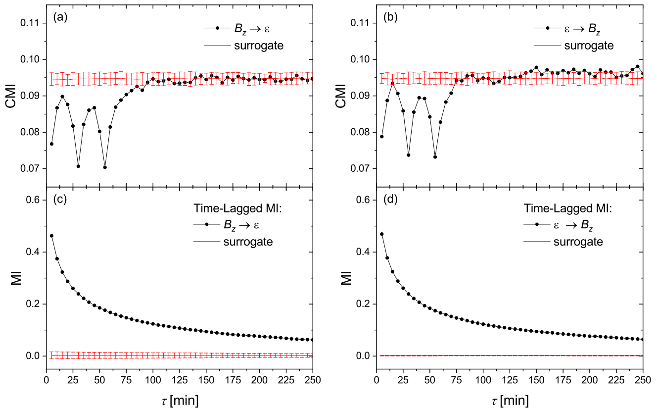
Figure 2. The conditional mutual information (CMI) (Equation (13)) obtained from the time series of B_z and \epsilon , for the information flow directions of (a) B_z \rightarrow \epsilon and (b) \epsilon \rightarrow B_z . The corresponding time-lagged mutual information (MI) between these two variables are represented in (c,d), respectively. The red lines and error bars represent mean and \pm 2 standard deviations for a set of 100 circular time-shifted surrogates.
