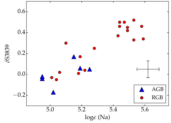
Figure 8. \delta S3839 (excess CN index values) versus Na abundances for stars in both our M 4 HERMES and AAOmega samples. \delta S3839 values are the distance a star is above the green trend-line in Fig. 7. The error bar represents typical uncertainties. Note that for two stars (25133 and 17999) only low-resolution spectra were observed, and they are therefore not included in this plot.
