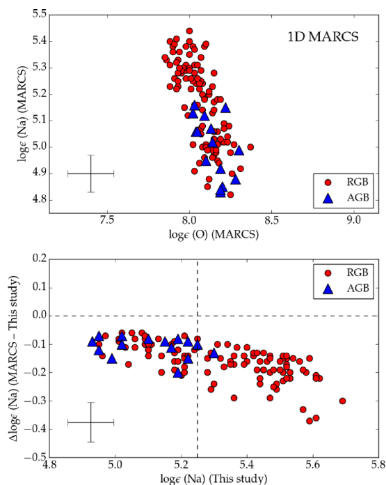
Figure 20. Top panel: Na and O abundances for each star in our M4 sample, determined using the BALDER code with the 1D MARCS grid of stellar atmospheric models (see Section 6.3 for details). Error bars indicate our total abundance uncertainties (Table 7). Bottom panel: The star-to-star differences in Na abundance as determined using (i) the BALDER code with the 1D MARCS grid and (ii) PHOBOS v2 with the 1D ATLAS9 grid of atmospheric models. Error bars indicate our total uncertainty in Na abundance. The dashed vertical line is at \log \epsilon(\text{Na}) = 5.25 , see Section 6.3 for details. Note that the stellar parameters from Table 3 were used for all determinations.
