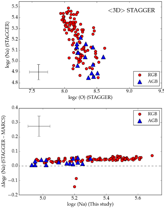
Figure 21. Top panel: Na and O abundances for each star in our M 4 sample, determined using the non-LTE BALDER code with the (3D) STAGGER-grid of stellar atmospheric models (see Section 6.3 for details). Error bars indicate our total abundance uncertainties (Table 7). Bottom panel: The star-to-star differences in Na abundance as determined using the non-LTE BALDER code with (i) the 1D MARCS and (ii) the (3D) STAGGER-grid of atmospheric models. The two outlying stars with negative differences are the two brightest stars in our sample, and were outside the STAGGER-grid by \sim 1.0 dex in \log g . Error bars indicate our total uncertainty in Na abundance.
