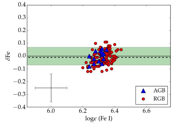
Figure 4. Fe abundances for this study. Here, ionization difference ( \delta\text{Fe} = \log_{\epsilon}(\text{Fe I}) - \log_{\epsilon}(\text{Fe II}) ) is plotted against \log_{\epsilon}(\text{Fe I}) abundance to highlight departures from LTE in Fe I, and the similarity between the Fe abundances of the AGB and RGB. The error bar indicates typical 1\sigma total uncertainties in individual abundances (i.e. the line-to-line uncertainties and the 1\sigma atmospheric sensitivity uncertainties added in quadrature), while the black dashed line represents the sample average \delta\text{Fe} value of -0.01 . The shaded green region indicates the non-LTE uncertainties quoted in Amarsi et al. (2016b, \pm 0.05 dex), around the expected \delta\text{Fe} value ( +0.00 dex, solid black line) from our non-LTE test (see Section 2.3).
