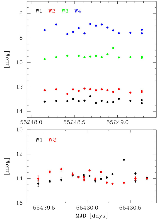
Figure 5. WISE light curves of VVV-WIT-04 within about 1 d coverage. Top panel: 2010 February data. Bottom panel: 2010 August data. For some data points, especially in the top panel, the error bars are smaller than the symbols.
